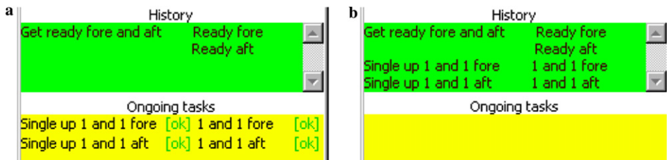
Fig. 9. Completed threads being added to history.
