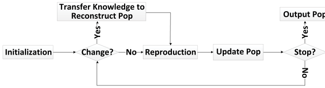
Fig. 3. Flow chart of KTDMOEA.
