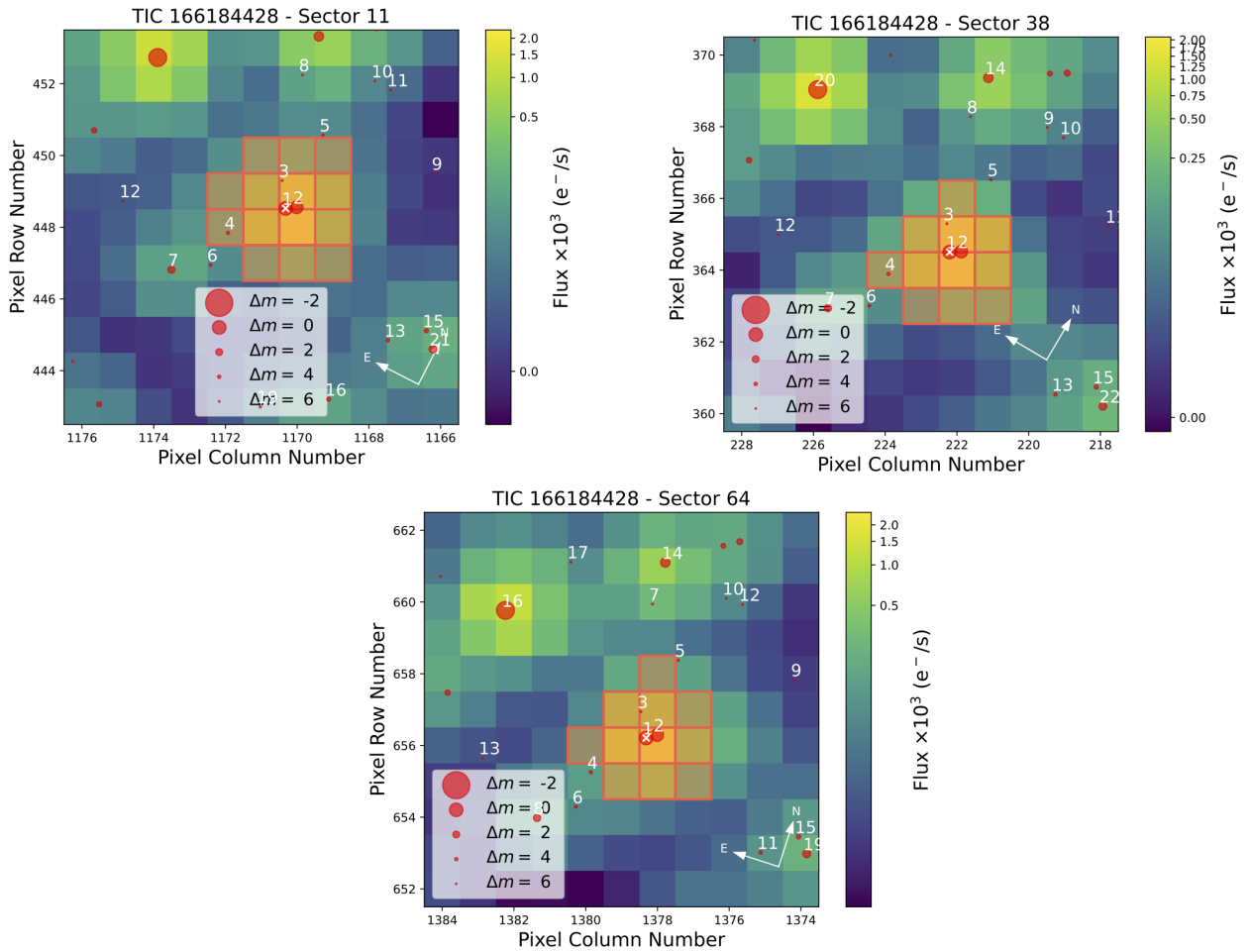
Fig. 4. TESS Target Pixel Files showing the custom apertures used to extract the photometry of TOI-4336 A b in this work for Sectors 11, 38, and 64.
