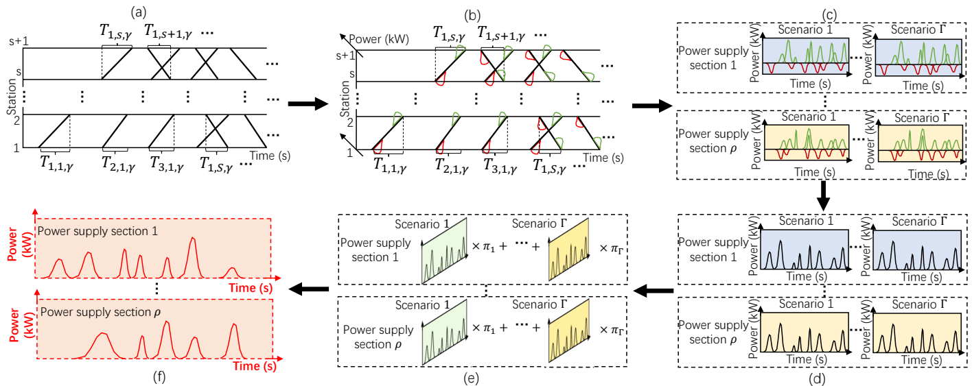
Fig. 21. The procedure to obtain the expected time-variant regenerative braking power distribution of the metro system: (a) Simulate the timetable of each scenario using T^\gamma following the base timetable of the studied system; (b) Simulate the power distribution of each scenario of the studied system (The red lines and green lines are the power profiles of the trains: red lines underneath the station-time plane represent the power consumed by trains, and green ones over the station-time plane represent the regenerative braking power); (c) Calculation of the time-variant net power values of all scenarios for all power supply sections; (d) Time-variant available regenerative braking power distribution of all scenarios for all power supply sections; (e) Calculation of the expected value based on all scenarios for all power supply sections; (f) Expected time-variant available regenerative braking power distribution for all power supply sections.
