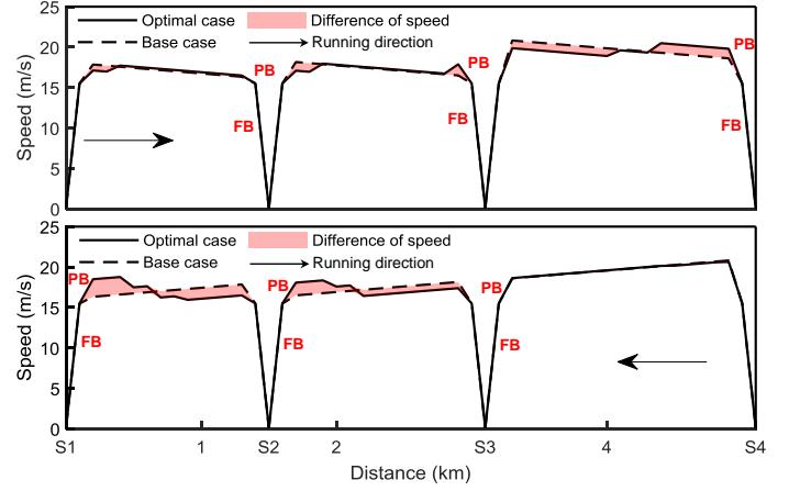
Fig. 13. The comparison between the optimal trajectory resulting from the proposed method (Optimal case) and the base trajectory from the case without the utilization of regenerative braking energy of other trains (Base case).
