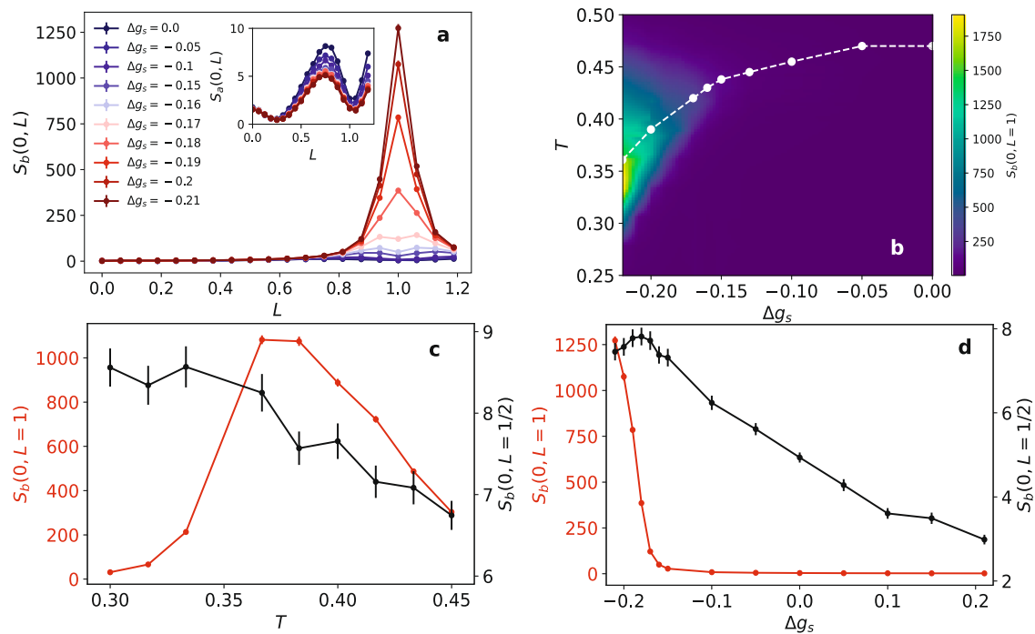
Fig. 4 | Theoretical CDW structure factors based on a non-linear sigma model. a The CDW structure factor at the in-plane wave vector of the b -CDW peaks as a function of L for T = 0.383 and various levels of the change in the CDW-mass, \Delta g_s , that models the effect of a axis compression. The inset depicts the CDW structure factor at the position of the a -peak under the same conditions. b The intensity of the L = 1b -CDW peak in the T - \Delta g_s plane. The broken line marks the superconducting
