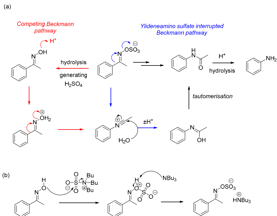
Scheme 2. (a) Proposed mechanism of this work (blue) versus acid-mediated Beckmann mechanism (red); and (b) mechanism of the O-oxime sulfation step.
