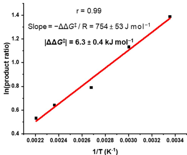
Fig. 6 Curtin-Hammett plot of macrocycle 2b , where 2b was synthesised at a range of temperatures ( T ) and the product ratio ( [\text{PM-2b}]/[\text{PP-2b}] ) determined by ^1\text{H} NMR spectroscopy.
