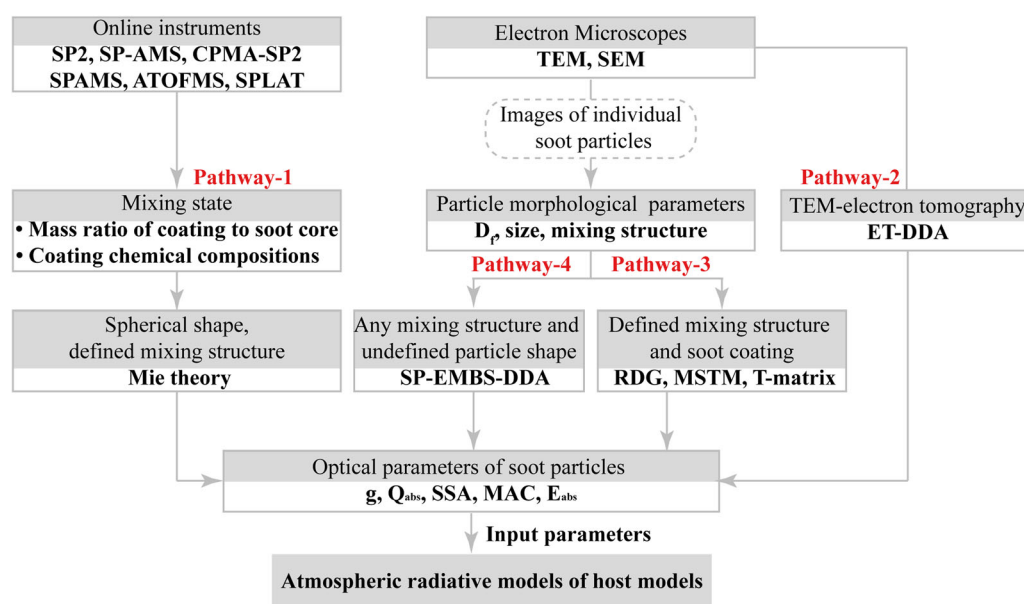
Fig. 6 | The different pathways from ambient measurements to atmospheric radiate models of soot (i.e., black carbon) aerosols. Pathway-1 was acquired from refs. 14, 27, 108, 114, 115, 119, 169,180. Pathway-2 was acquired from ref. 74. Pathway-3 was acquired from refs. 37,110 and Pathway-4 was acquired from refs. 13, 38, 56, 71,77.
