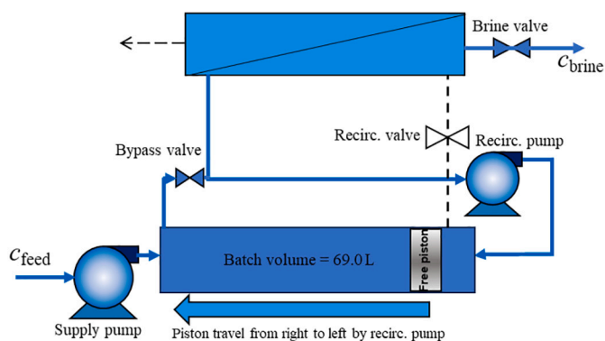
Fig. 2. Schematic of the free-piston batch RO, a) pressurization, and b) purge-and-refill phase. The phases involve switching three on-off valves. In the pressurization phase, the bypass and brine valves are closed while the recirculation valve remains open. Conversely, in the purge-and-refill phase, the bypass and brine valves are open, and the recirculation valve is closed. For more details refer to [27]. Solid and dashed lines represent flow and no flow respectively.
