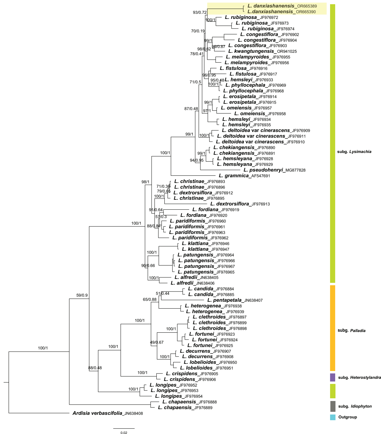
Figure 1. Phylogenetic tree of Lysimachia danxiashanensis and related species generated by Bayesian Inference (BI) of the combined dataset (ITS, rbcl ). Bootstrap values of the ML and BI posterior probabilities are shown along the branches. The new species in yellow shaded area, green indicates subgen. Lysimachia , orange is subgen. Palladia , purple is subgen. Heterostylandra and grey is subgen. Idiophyton . Blue indicates outgroup, Ardisia verbascifolia .
