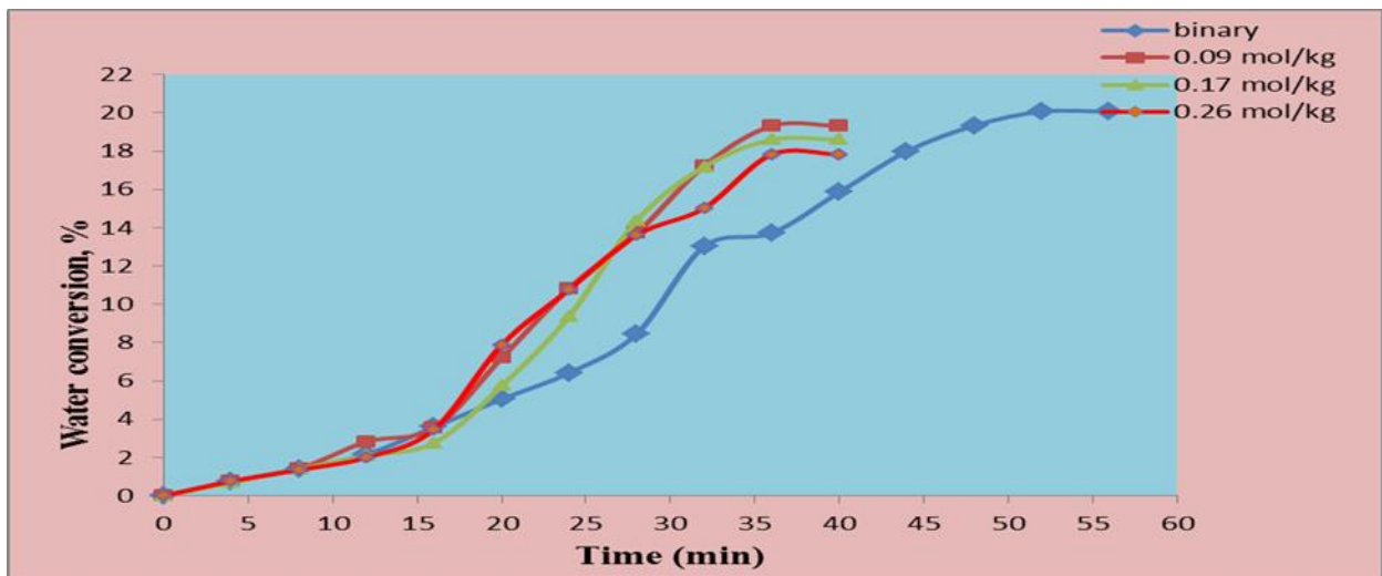
Figure 23: The water to hydrate conversion as function with time for the ternary system in the presence of sodium chloride.
