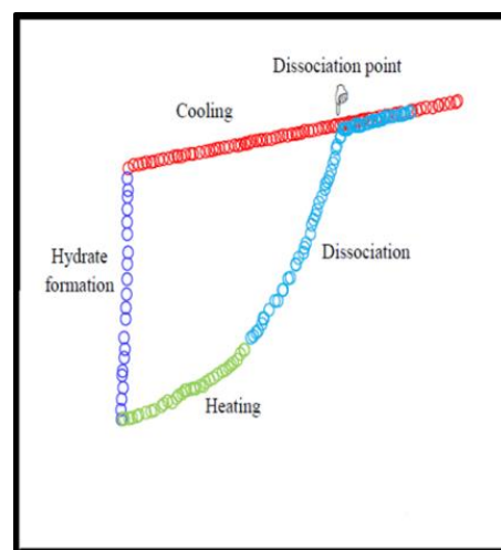
Figure1: Isochoric search technique [15]
