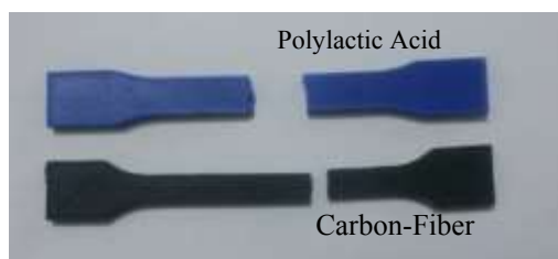
Figure 10: The specimens of Poly lactic Acid and Carbon fiber after testing
