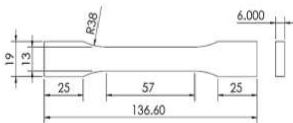
Figure 5: Poly-lactic Acid standard Tensile Specimen (All dimensions in mm).
