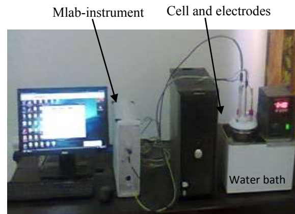
Figure 2: M-Lap Potentiostatic test collection
