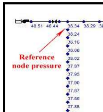
Figure (5). Farm level (separated pump stations) simulated sprinkler system layout
