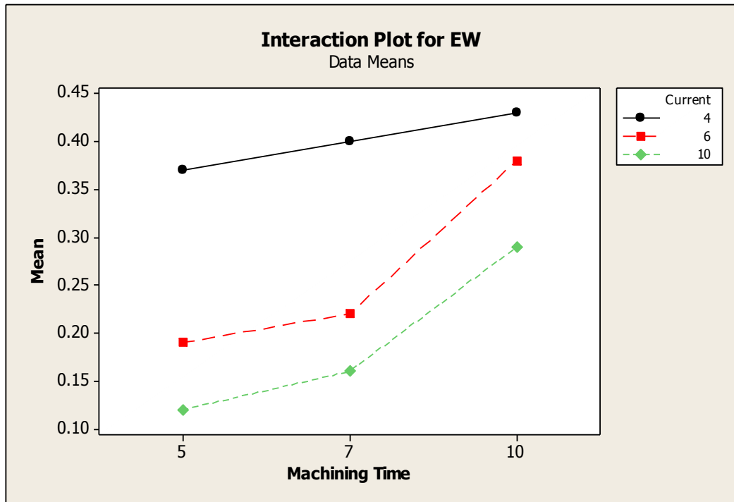
Figure (4) Interaction plot for Electrode Wear (EW).
