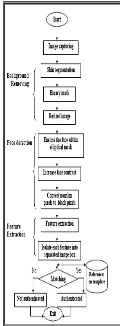
Figure (2) The proposed system flowchart
