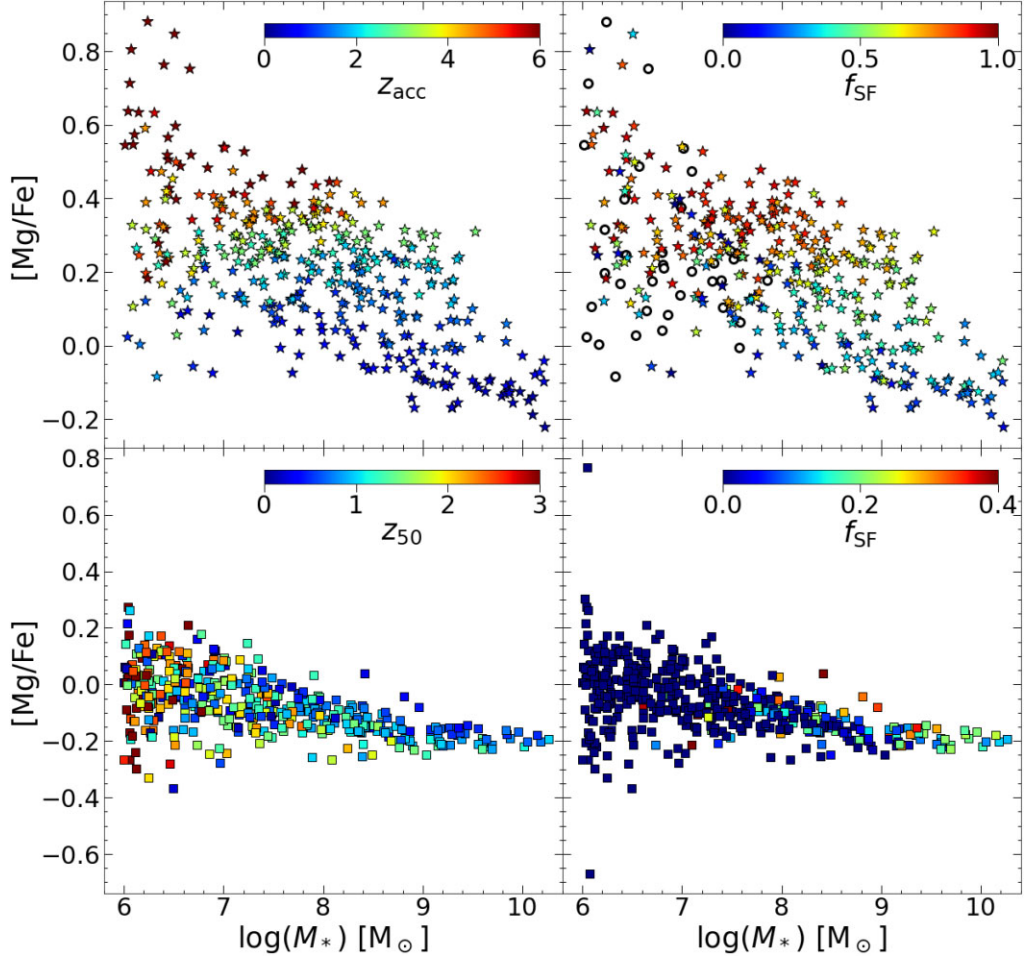
Figure 6. Top: [\text{Mg}/\text{Fe}] – M_* distributions for the disrupted populations, with values colour-coded by z_{\text{acc}} (left) and by f_{\text{SF}} at accretion (right). Systems with f_{\text{SF}} = 0 are shown with empty circles. A clear correlation of the scatter in [\text{Mg}/\text{Fe}] at fixed M_* is seen for the disrupted dwarfs, with both z_{\text{acc}} and f_{\text{SF}} . Bottom: The same distributions for the surviving dwarfs, colour-coded by z_{50} (left) and by f_{\text{SF}} at z = 0 (right). The correlations of the scatter with these parameters are much weaker in this case.
