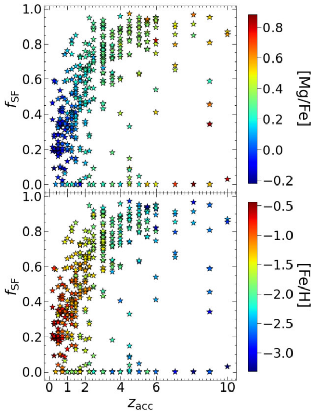
Figure 7. Star-forming gas fraction, f_{\text{SF}} , versus redshift of accretion, z_{\text{acc}} , for disrupted dwarfs. Values are colour-coded by [\text{Mg}/\text{Fe}] (top) and by [\text{Fe}/\text{H}] (bottom), respectively. The f_{\text{SF}} values tend to decrease with redshift, with a sharp turnover around z_{\text{acc}} \approx 4 . Before this redshift, there is a considerable scatter in the relation between these parameters, however after this redshift the two parameters correlate well.
