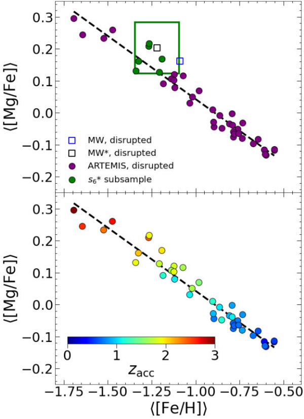
Figure 8. Top: The \langle [Mg/Fe] \rangle – \langle [Fe/H] \rangle relation of disrupted populations in the simulations (filled circles). Symbols represent the mass averages of each disrupted population in the 42 simulated MW-mass systems. \langle [Mg/Fe] \rangle anticorrelates with \langle [Fe/H] \rangle . The best fit is a linear relation with a slope of -0.40 \pm 0.015 . The blue and black squares correspond to the samples of disrupted dwarfs in the MW: including I’itoi and Sagittarius (MW sample) and excluding them (MW* sample), respectively. The six closest populations to the MW* data in this relation are shown with green circles and called the ‘ s_6^* subsample’. Bottom: Same relation as above, colour-coded by the \langle z_{acc} \rangle of each disrupted population. There is a strong anticorrelation between \langle z_{acc} \rangle and \langle [Fe/H] \rangle (recently accreted populations are more metal-rich) and a strong correlation between \langle z_{acc} \rangle and \langle [Mg/Fe] \rangle (recently accreted populations have lower [Mg/Fe] abundances).
