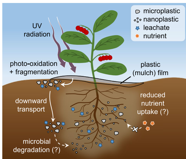
Fig. 3 Plastics in agricultural environments. Plastic mulch is photo-oxidised and fragmented due to exposure to UV radiation and mechanical stressors. This process releases various sized plastic fragments (grey) and leachates (blue stars). These degradation products are dispersed downwards into the soil, where they are not subjected to further photo-oxidation and thus tend to accumulate. The fate of buried plastics is subject to considerable uncertainties. Potentially, microbial processes can degrade plastics, contributing to its removal. Plastic fragments may also interfere with plant nutrient uptake. Full arrows indicate processes that are well established; dashed arrows show processes whose occurrence is less certain
