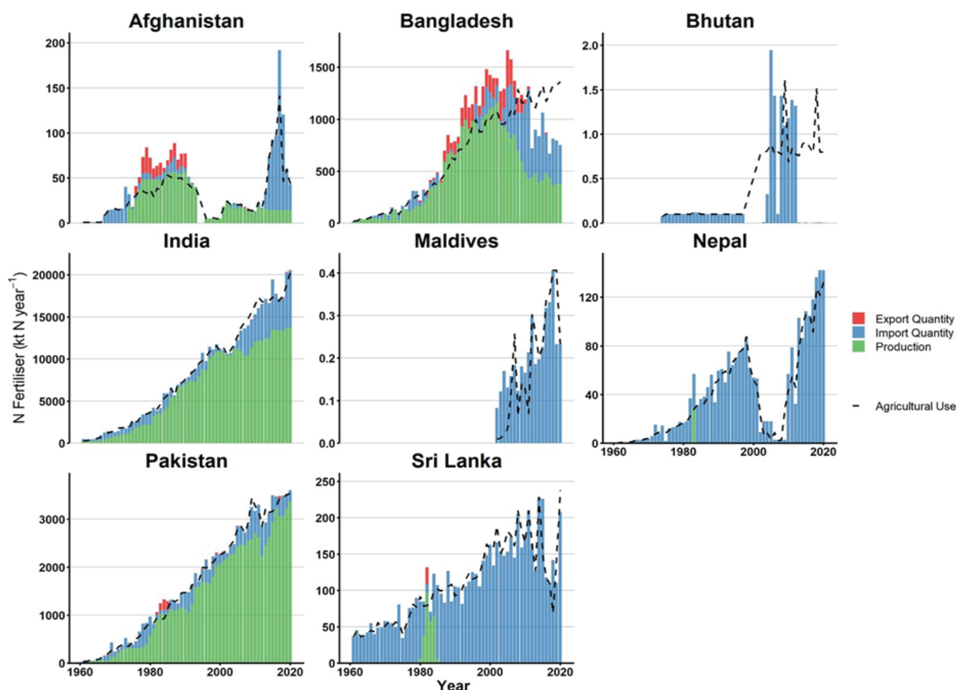
Figure 7. Production, import, export and use of synthetic N fertiliser (kt) by South Asia countries from 1960 -2020. Stacked graphics showing the sum of the first three components, compared with estimated agricultural use, plotted using data reported by FAOSTAT 2022. Differences between production plus import minus export and agricultural use indicate uncertainties, changes in stored fertilizer and other N uses.
