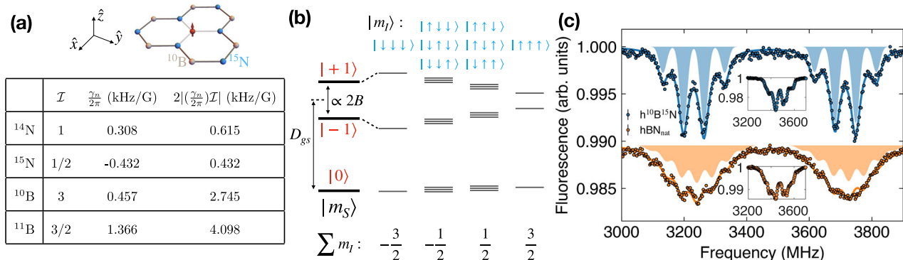
Fig. 1 V_B^- electron spin resonance spectra in isotopically distinct hBN samples. a Schematic of an individual V_B^- center (red spin) in an isotopically purified h^{10}\text{B}^{15}\text{N} crystal. \hat{z} is defined along the c -axis (perpendicular to the lattice plane) and \hat{x} and \hat{y} lie in the lattice plane, with \hat{x} oriented along one of the three V_B^- Nitrogen bonds. The table lists the nuclear spin quantum number ( I ), gyromagnetic ratio ( \gamma_n ), and overall electronic spin transition width ( \propto 2|\gamma_n I| ) of the four stable atomic isotopes in hBN. b Energy level diagram of the V_B^- electronic ground state coupled to the three nearest-neighbor ^{15}\text{N} nuclear spins ( I = \frac{1}{2} ) under an external magnetic
