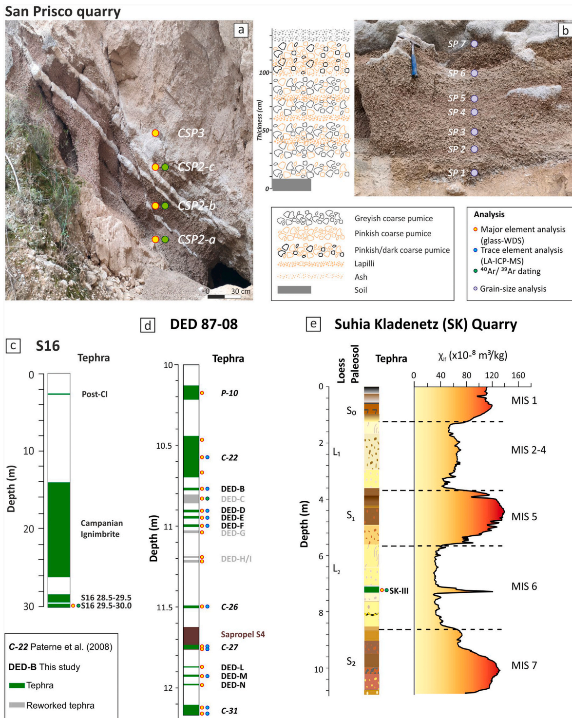
Fig. 2. a) and b) Photographs and stratigraphic log of the San Prisco sequence (41°05'31''N; 14°17'25''E, Campanian Plain; Fig. 1). a) CSP2 (a, b and c) and CSP3 were sampled for EMPA and ^{40}\text{Ar}/^{39}\text{Ar} analyses. b) Samples SP1 to SP7 were sampled for grain-size analyses. Full dataset is provided in the Supplementary Material (S1 and S3). c) Simplified section of the core S16 (41°07'02''N; 14°01'23''E, Campanian Plain) investigated for the first time in this study; d) Simplified section of the marine core DED 87-08 (39°42'14''N; 13°34'93''E, Central Tyrrhenian Sea); e) Loess-paleosol succession of the Suhia Kladenetz Quarry (43°27'24.0''N, 24°41'26.7''E; Central North Bulgaria, Lower Danube). For further details about the core DED 87-08 and Suhia Kladenetz Quarry successions the reader is referred to Paterne et al. (1988, 2008) and Jordanova et al. (2022), respectively.
