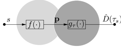
Figure 2: A framework for prediction of the incurred distortion, D(\tau_s) = \delta(s, \mathcal{Q}_\tau(s)) , when coding a random vector s , using coding template \tau . A dimension reducing property vector extraction, f(\cdot) , is followed by a distortion prediction, g_\tau(\cdot) .
