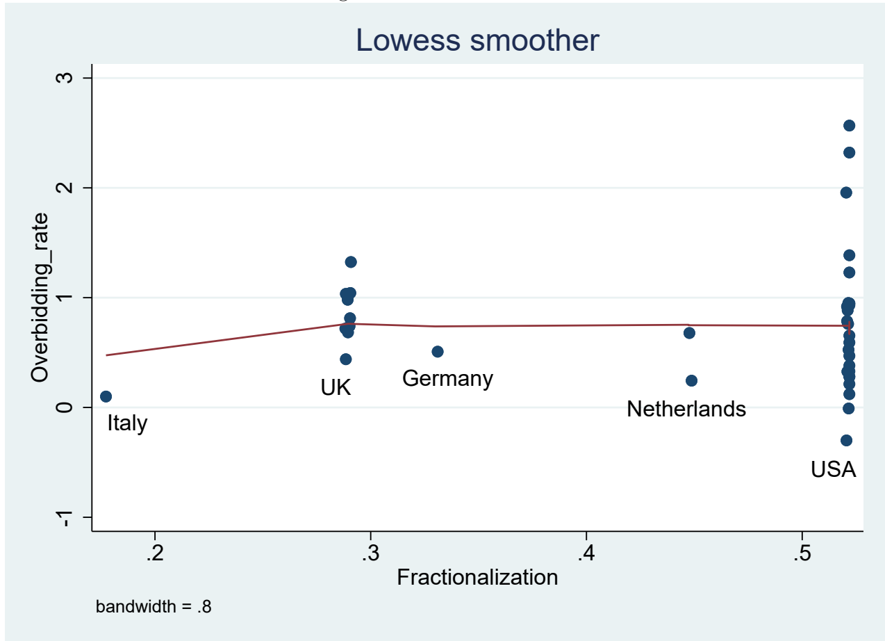
Figure 1: Lowess smoother
