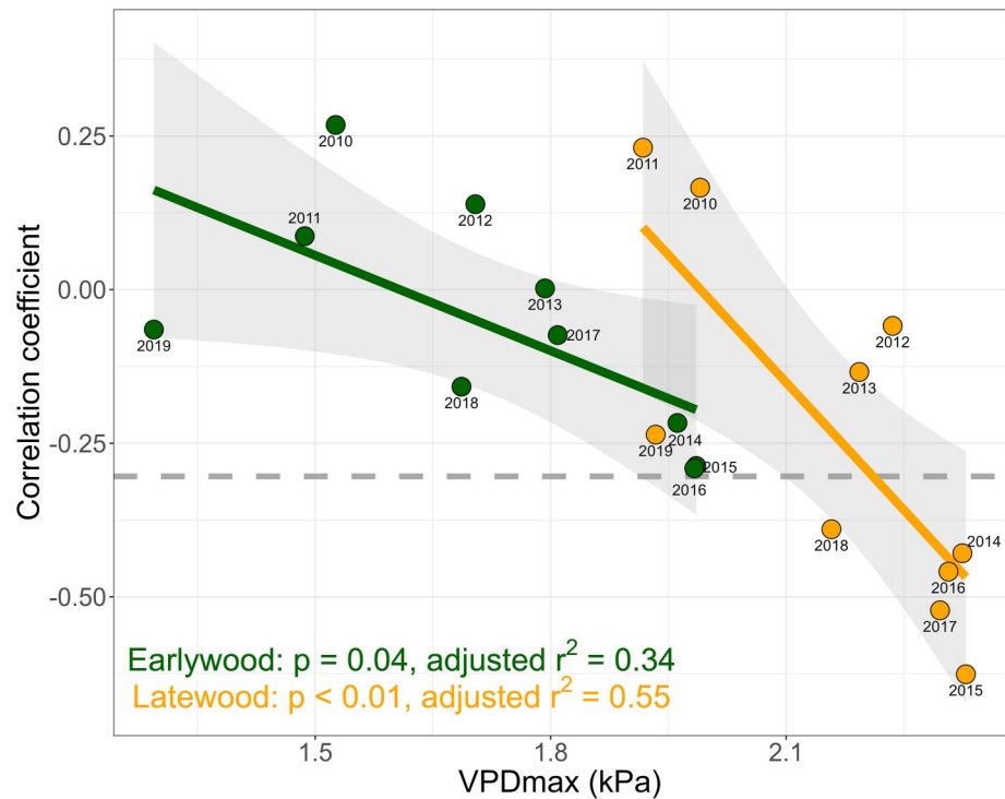
Figure 3. Correlations between annual values of \delta^{18}\text{O} and \Delta^{13}\text{C}_{\text{res}} ( \Delta^{13}\text{C}_{\text{res}} ) as a function of maximum vapor pressure deficit ( \text{VPD}_{\text{max}} ). Pairs of \Delta^{13}\text{C}_{\text{res}} and \delta^{18}\text{O} values for all trees at all sites within the lower Santa Clara River, California (42 trees) were compared to calculate annual values of correlation, with each point representing a year from 2010 to 2019. Correlations were calculated separately for earlywood (green) and latewood (orange). Values of \text{VPD}_{\text{max}} were aggregated across all sites and averaged over the months of February–June for the earlywood comparison and March–September for the latewood comparison. Separate trendlines are displayed for earlywood and latewood with standard error shaded. Horizontal dashed line depicts the threshold below which all points show a significant correlation between \Delta^{13}\text{C}_{\text{res}} and \delta^{18}\text{O} ( p < 0.05 ).
