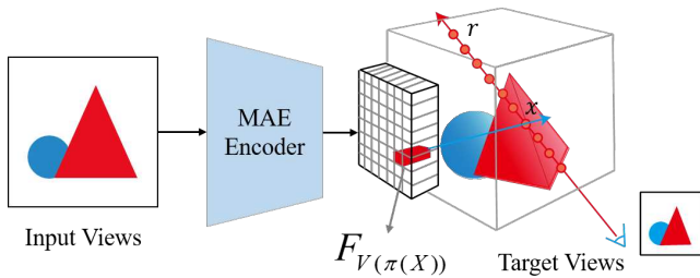
Fig. 3 Image feature extraction. Given the input image, F_{V(\pi(X))} is extracted with the feature extraction network.
