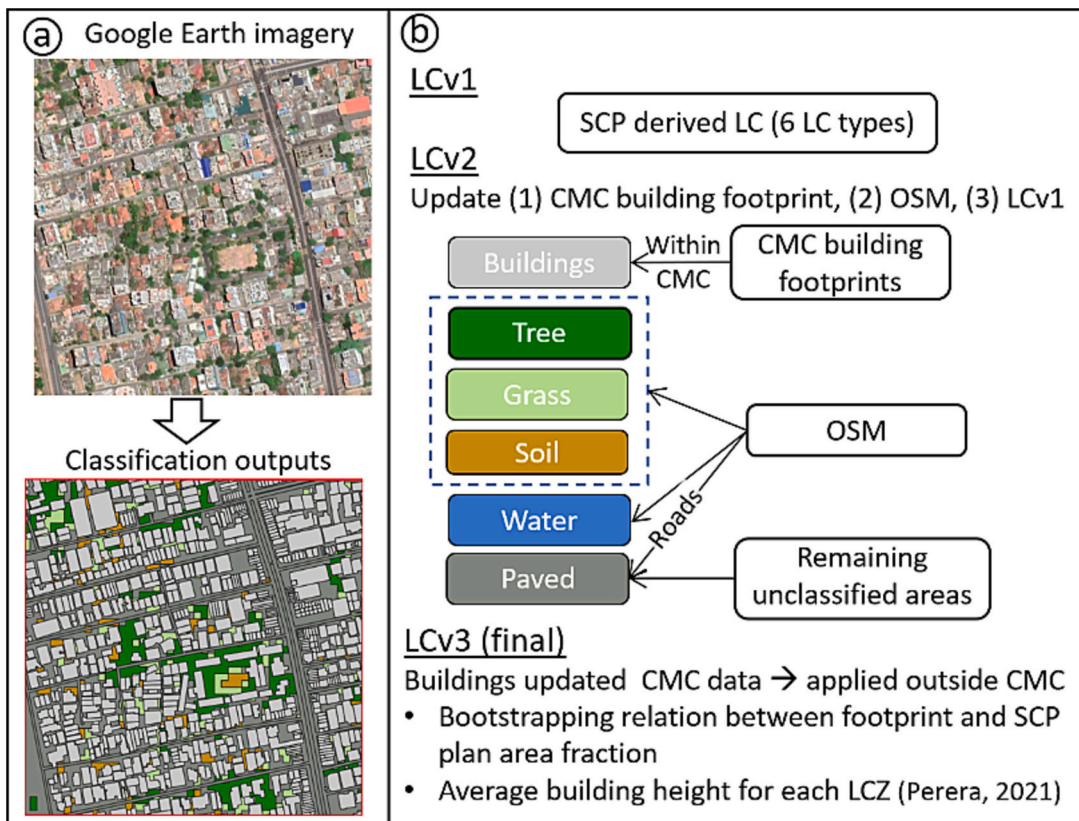
Fig. 2. Land cover fraction calculation (b) procedures and (a) example outputs.
