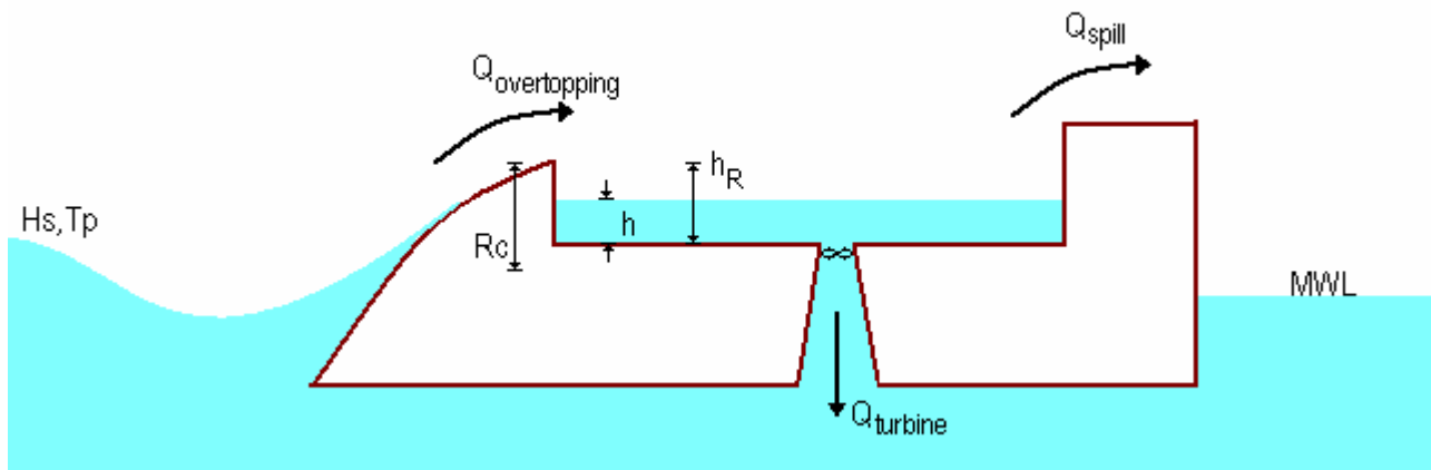
Schematic of flows on Wave Dragon
