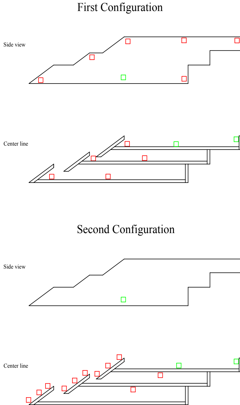
Figure 12. The approximate position of the 14 pressure cells are marked with red and green. The three marked with green are not moved from one configuration to another. They are used to compare the results from the two configurations.
