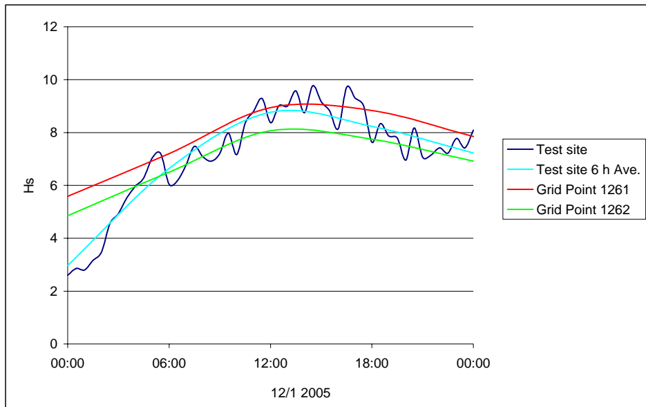
Figure 3. Comparison of H_s .
