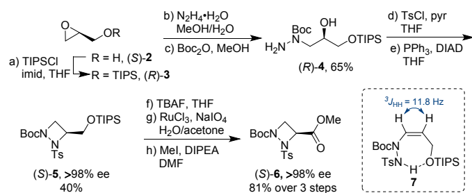
Scheme 1. Synthesis of ( S )-1,2-diazetidene-3-carboxylic acid building block ( S )- 6 .
