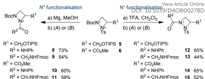
Scheme 2. Orthogonal functionalisation of N v and N δ in 5 and 6 .
