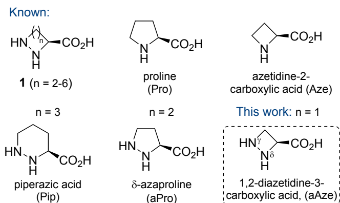
Figure 1. Cyclic amino and \alpha -hydrazino acids.
