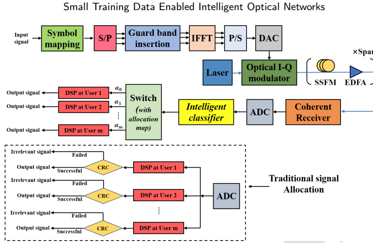
Figure 2: Block diagram of the proposed optical system model where signals are classified by the intelligent classifier and forwarded to their target users, thereby easing user-side processing compared to the traditional signal allocation method. S/P: serial to parallel; P/S: parallel to serial; DAC: digital-to-analog converter; ADC: analogue-to-digital converter; SSFM: split-step Fourier method; EDFA: erbium-doped fiber amplifier; Optical I-Q modulator: optical in-phase and quadrature modulator; DSP: digital signal processing; CRC: cyclic redundancy check.
