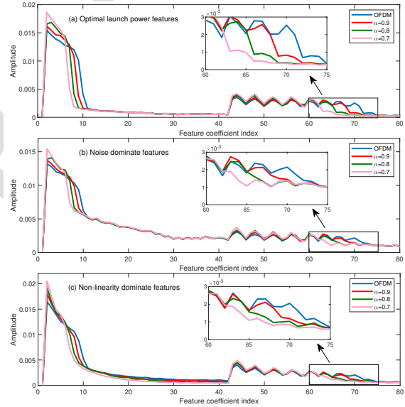
Figure 11: Signal feature illustration to explain the mechanism of wavelet scattering neural networks in non-orthogonal signal classification. (a) Features at optimal launch power. (b) Features when noise dominates. (c) Features when non-linearity dominates.
