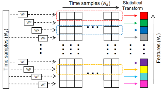
Figure 3: One-dimensional wavelet feature generation based on wavelet filtering (WF) and statistical feature dimensionality reduction.
