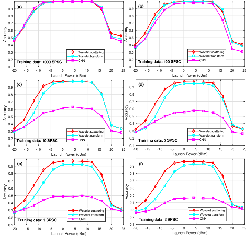
Figure 7: Classification accuracy of three signal classifiers when different training symbols per signal class (SPSC) values are considered.
