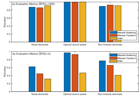
Figure 10: Evaluation of three signal classifiers under two training conditions: (a) Sufficient training dataset with SPSC = 1000 , and (b) Insufficient training dataset with SPSC = 2 .
