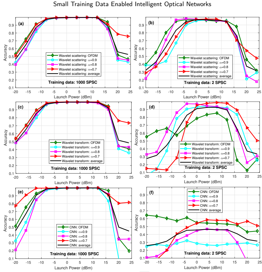
Figure 8: Classification accuracy of three signal classifiers for individual signal classes and the average accuracy considering training symbols per signal class (SPSC)=1000 and SPSC = 2 scenarios.
