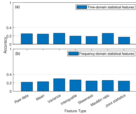
Figure 6: Classification accuracy of statistical feature-based SVM with SPSC = 1000 and 4 dBm launch power using (a) time-domain and (b) frequency-domain statistical features.
