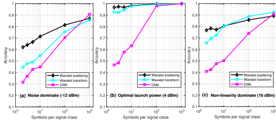
Figure 9: Evaluation of three signal classifiers under three extreme conditions: (a) Noise dominate, (b) Optimal launch power, and (c) Non-linearity dominate. The launch power level in each condition is given in parentheses.
