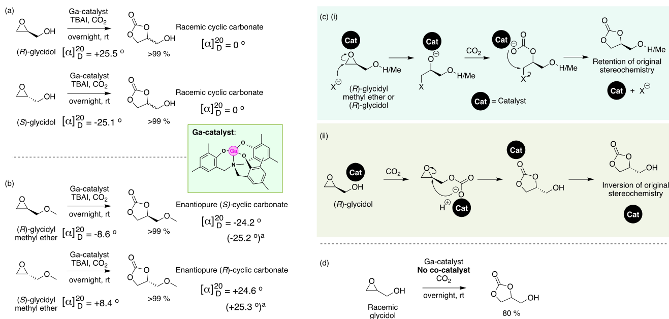
Scheme 3. (a) Cycloaddition of enantiopure ( R )- or ( S )-glycidol with \text{CO}_2 forming racemic cyclic carbonate product mixtures: loss of original stereochemistry. (b) Cycloaddition of enantiopure ( R )- or ( S )-glycidyl methyl ether with \text{CO}_2 forming the enantiopure cyclic carbonate products: retention of original stereochemistry. (c) Mechanisms for retention and inversion of stereochemistry during cyclic carbonate synthesis from glycidol and glycidyl methyl ether. (d) Results obtained in the absence of co-catalyst (TBAI). Reaction conditions for all experiments: Substrate (10.0 mmol epoxide), Gallium catalyst (0.5 mol%), TBAI (2.0 mol%), 8.0 bar \text{CO}_2 , rt, overnight. a Optical rotation values obtained from commercially available samples with an enantiomeric excess (ee) of >99%.
