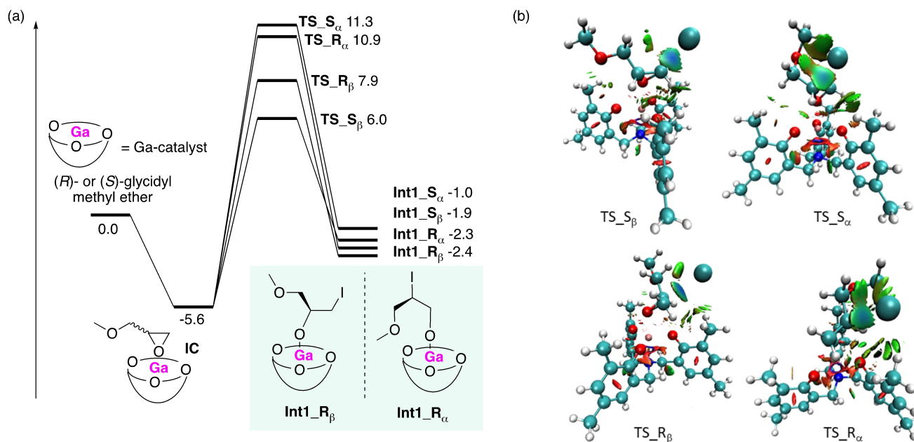
Figure 2. a) Calculated free energy surface ( \Delta G_{298K} ), \omega B97M-V/def2-tzvpv, for the Gallium catalyst (Ga-Catalyst)/TBAI assisted ring-opening of ( R )- and ( S )-glycidyl methyl ether. b) NCI plots for calculated transition state structures.
