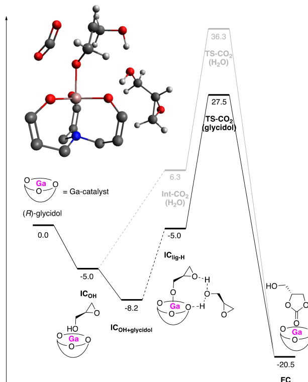
Figure 3. Calculated free energy surface ( \Delta G_{298K} ), \omega B97M-V/def2-tzvpv, for the Gallium catalyst (Ga-catalyst)/glycidol cluster assisted cycloaddition of \text{CO}_2 and ( R )-glycidol. Phenolate groups on the calculated structure have been omitted for clarity.
