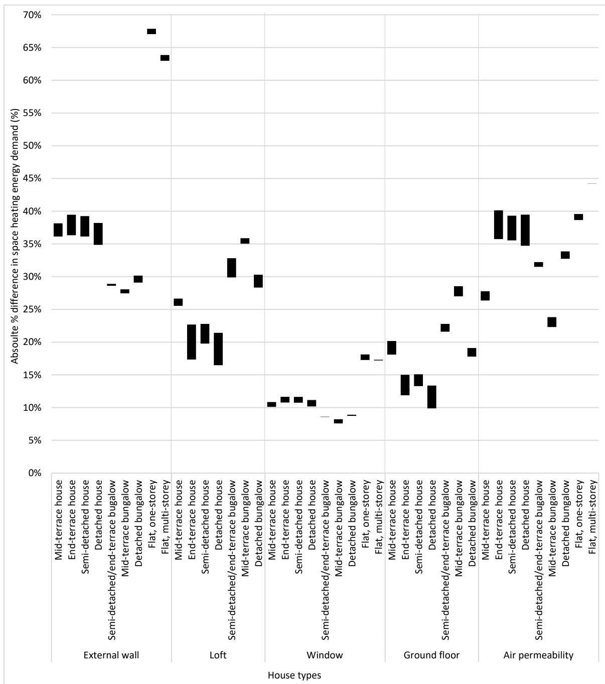
Figure 9. Effect of selected lower and upper bounds on fabric uncertainty for all the 32 archetypes; the bar represents data from different numbers of bedrooms.
