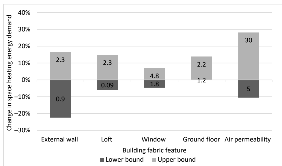
Figure 6. Percentage change relative to the base case for combined lower and upper bounds for five building fabric features, with the data labels showing the input parameters (U-values and air permeability) in Table 3.
