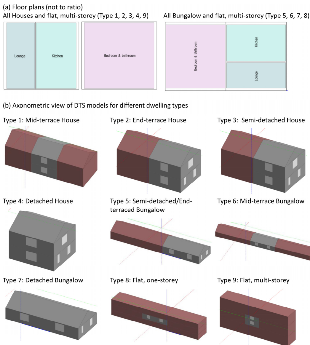
Figure 2. (a) Floor plan and (b) DTS models of three-bedroom building archetype for different dwelling types.
