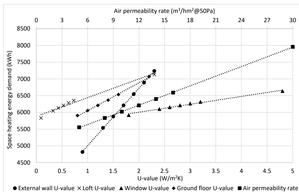
Figure 4. Space heating energy demand for the five perturbations, and lower and upper bounds (defined in Table 3) for 15% WWR semi-detached three-bedrooms house.
