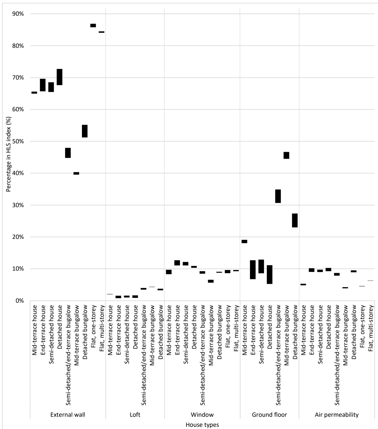
Figure 8. Significance of fabric sensitivity on model accuracy for all the 32 dwelling archetypes; the bar represents data from different numbers of bedrooms.
