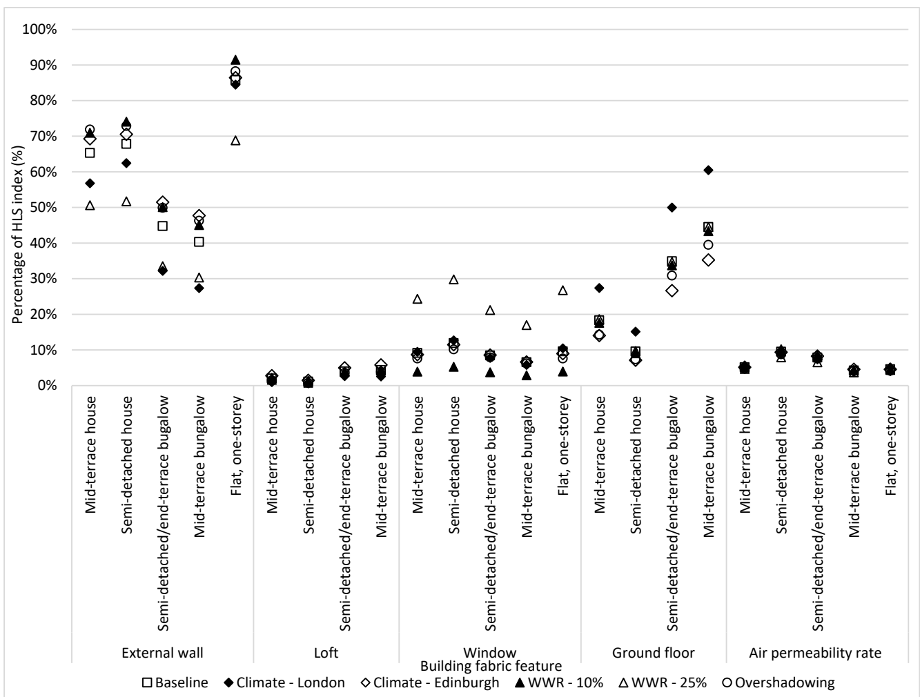
Figure 11. Significance of fabric sensitivity with varying climates, WWRs, and overshadowing compared to baseline.
