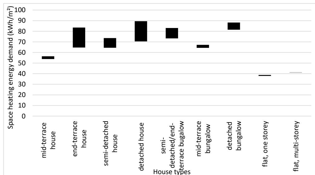
Figure 7. Space heating energy demand for different house types; the bar represents data from homes with different numbers of bedrooms (one to four bedrooms).
