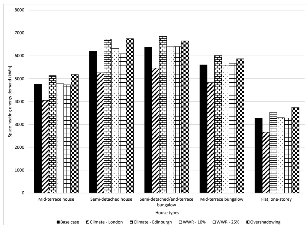
Figure 10. Variation in space heating energy demand for selected house types when different parameters are alternated compared to the baseline.
