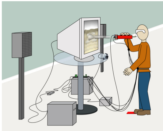
Figure 1. Setup of the virtual reality flute. A physical interface controls the flute physical model together with its visualization.
