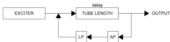
Figure 2. Block diagram of the flute physical model, based on digital waveguides. LP represents the low-pass filter simulating losses, while AP represents the all pass filters used to simulate changes in dimensions of the instrument.
