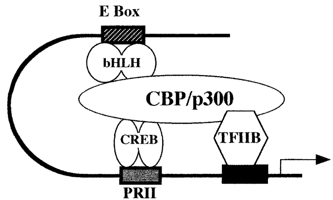
FIG. 5. Schematic showing the possible mechanism by which CREB or related cAMP-inducible proteins and bHLH proteins activate the transferrin promoter. An optimal promoter activation in response to FSH may require the interaction between bHLH and CREB-like proteins through transcriptional coactivators such as CBP and p300. The activation of the mTf by FSH may be due to the formation of ternary complex involving the binding of bHLH and CREB-like proteins to E-box and PRII, respectively, and transcriptional coactivators such as CBP and p300. The CBP/p300 may also bind to the components of the basal transcriptional machinery such as TFIIB. The intrinsic histone acetyl transferase activity of CBP/p300 and the spatial orientation of PRII and E-box around histones may cause DNA bending. The bending and relaxation of the chromatin structure may facilitate an organization that, in turn, facilitates the interaction of bHLH proteins, CREB, and CBP/p300.
