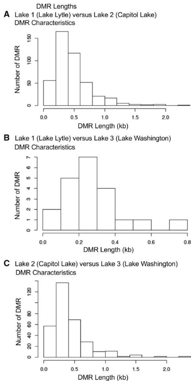
Figure 6: the cDNA DMR lengths. All cDNA DMRs at a P-value threshold of P < 1e-05 . (A) Lake 1 (Lytle Lake) versus Lake 2 (Capitol Lake). (B) Lake 1 (Lytle Lake) versus Lake 3 (Washington Lake). (C) Lake 2 (Capitol Lake) versus Lake 3 (Washington Lake)
