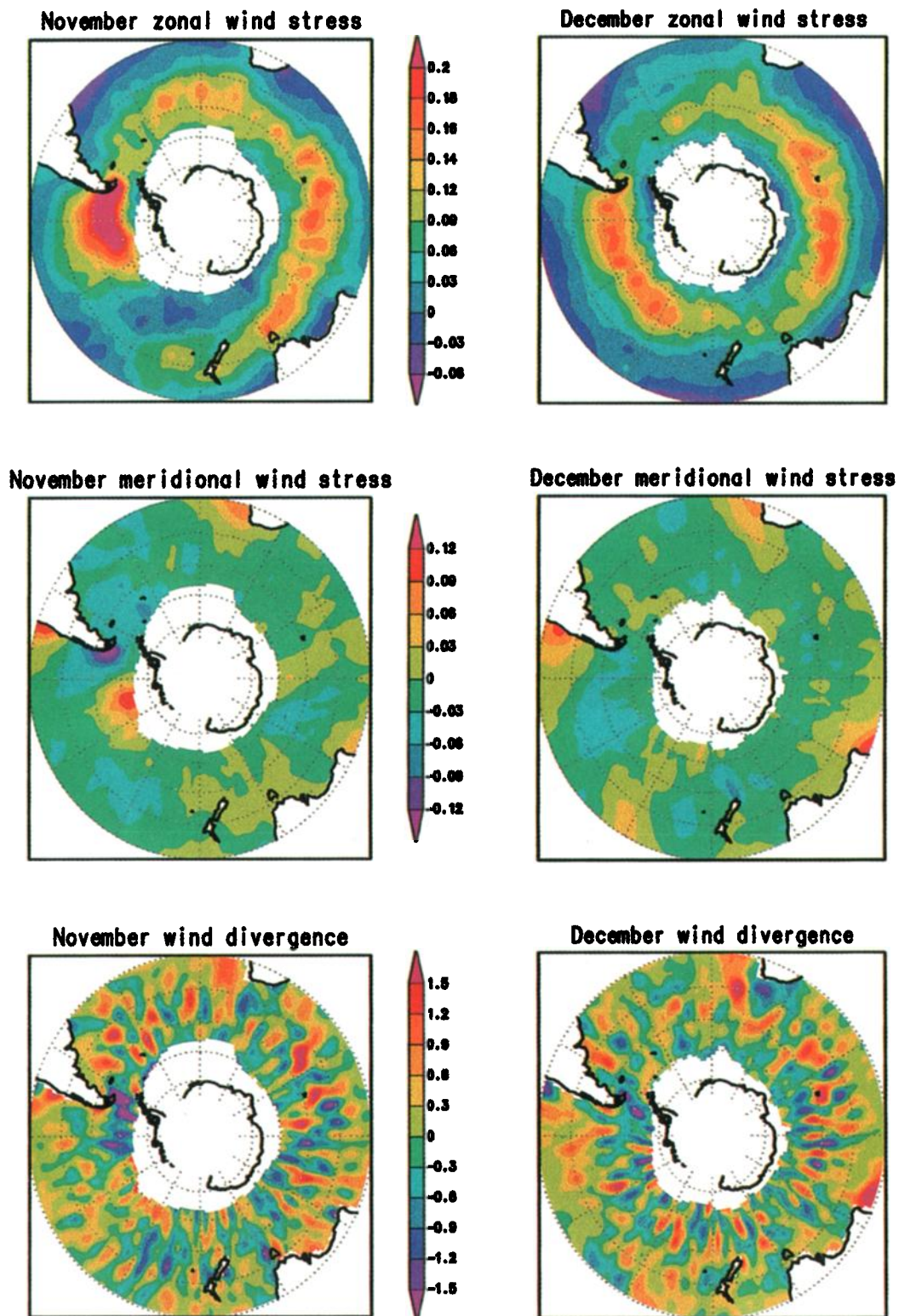
Plate 5. The monthly mean NSCAT \tau_x , \tau_y , and wind stress divergence for November and December, 1996.
