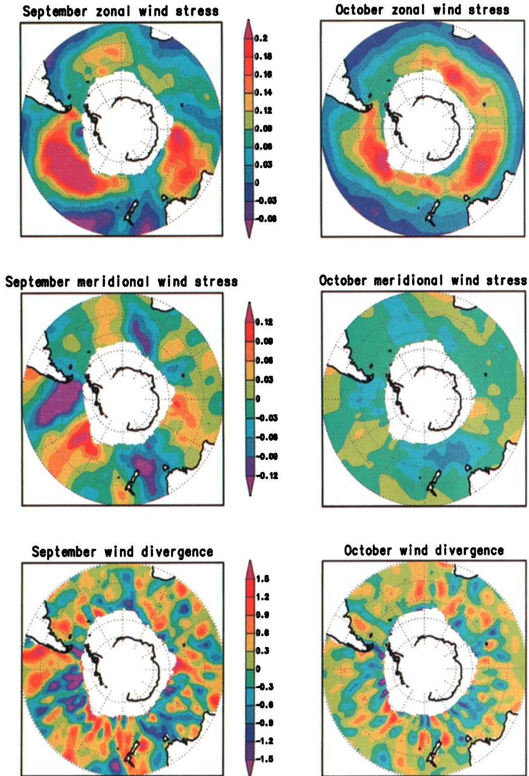
Plate 4. The mean NSCAT zonal wind stress \tau_x , meridional wind stress \tau_y and wind stress divergence for September and October, 1996. The September monthly mean is calculated from the available data between September 15 and September 31.
