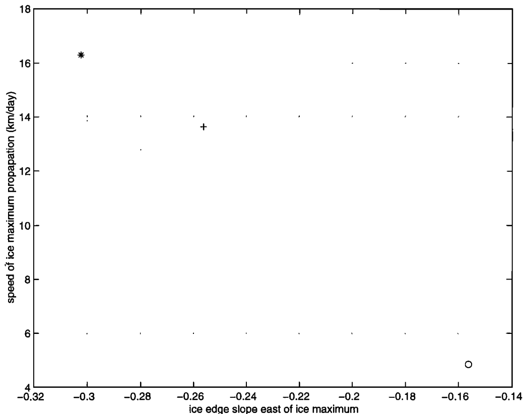
Figure 7. Mean propagation speed of sea ice maximum in the central Indian Ocean (circle), east of the Ross Sea (plus sign) and eastern Weddell Sea (asterisk) as a function of mean ice edge slope east of the ice maxima. Both the ice maximum propagation speed and ice edge slope are derived from monthly wind and sea ice data, and then averaged over September and October, 1996.
