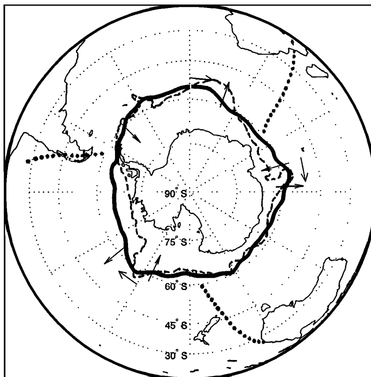
Figure 6. Schematic geostrophic winds (arrows) introduced by the sea ice distribution near the three ice-extent maxima. Solid line is the SIE in October 1996. Dashed line is the geopotential height anomaly 0.35 (10 \text{ J kg}^{-1}) contour at 50 dB with respect to 1000 dB reprinted from Deep-Sea Research , 42, Orsi et al. , On the meridional extent and fronts of the Antarctic Circumpolar Current, Page 645, Copyright (1995), with permission from Elsevier Science. Dotted lines are the positions of the ridges of standing wave number 3 from van Loon and Jenne [1972].
