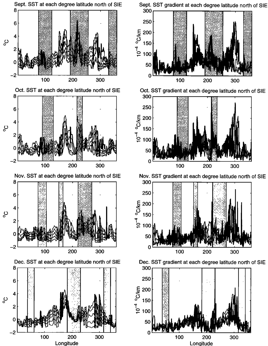
Figure 5. (left column) Sea surface temperature and (right column) meridional gradient of the sea surface temperature at every degree of latitude north of the ice edge up to 5^\circ of latitude for September, October, November, and December. Shaded areas indicate southerly winds north of the SIE in the monthly mean wind stress fields, while open areas indicate northerlies north of the SIE.
