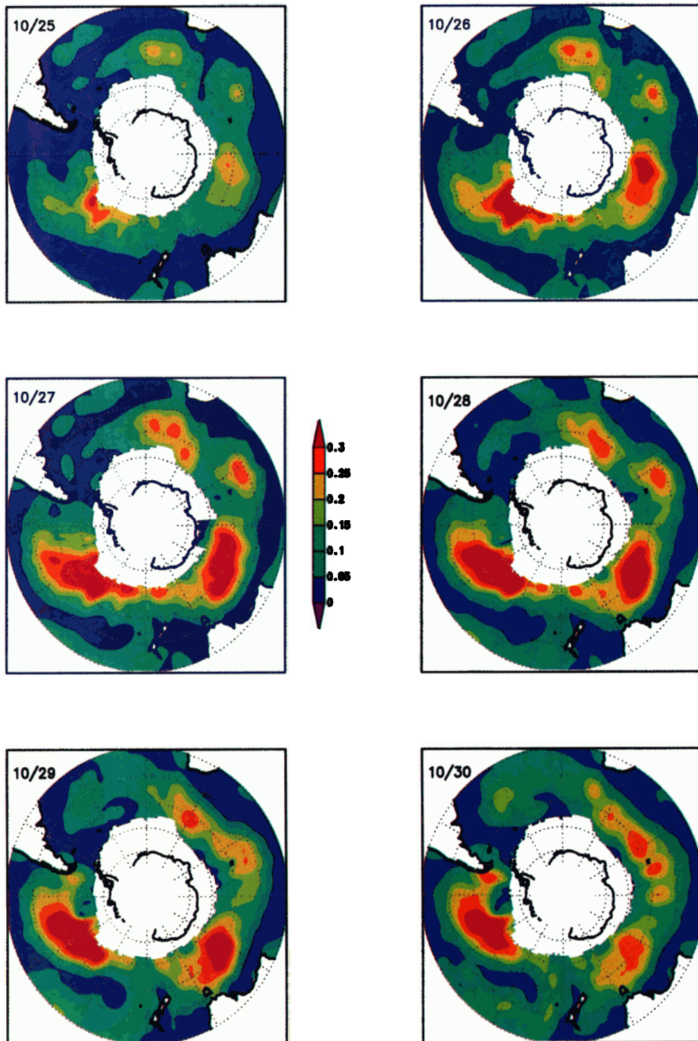
Plate 1. NASA scatterometer (NSCAT) wind stress magnitude from October 25 to October 30, 1996. A storm initiated in the marginal ice zone (MIZ) north of the Ross Sea ice maximum on October 25 and developed into a large storm event in the southeastern Pacific through October 30. Another storm started northeast of the Indian Ocean ice maximum on October 26 and spun off into the Antarctic Circumpolar Current region south of Australia through October 29.
