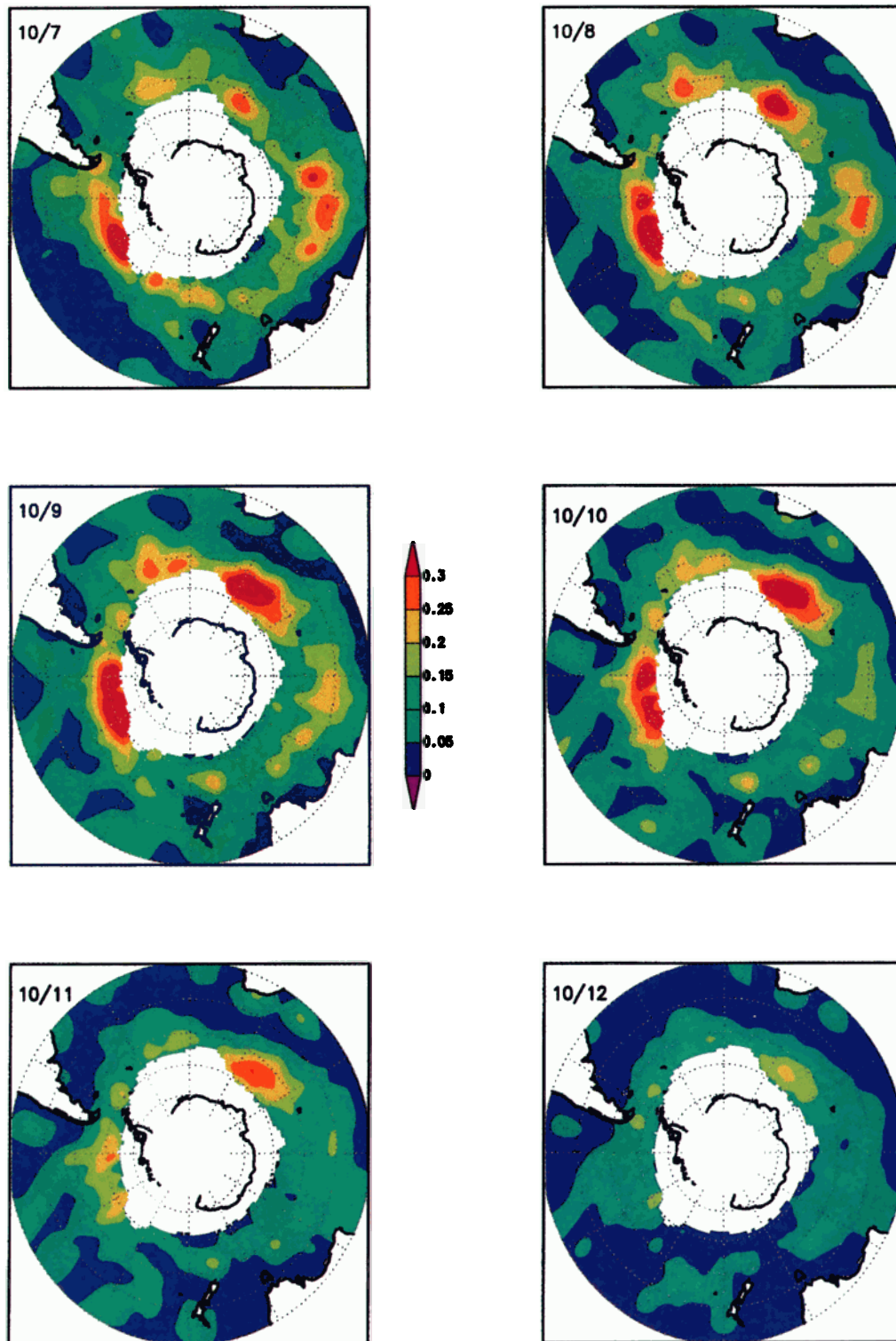
Plate 2. NSCAT wind stress magnitude from October 7 to October 12, 1996. A storm started east of the Ross Sea ice maximum on October 7 and lasted 4 days. Another storm started northeast of the Weddell Sea ice maximum on October 8 and also lasted 3 days.
