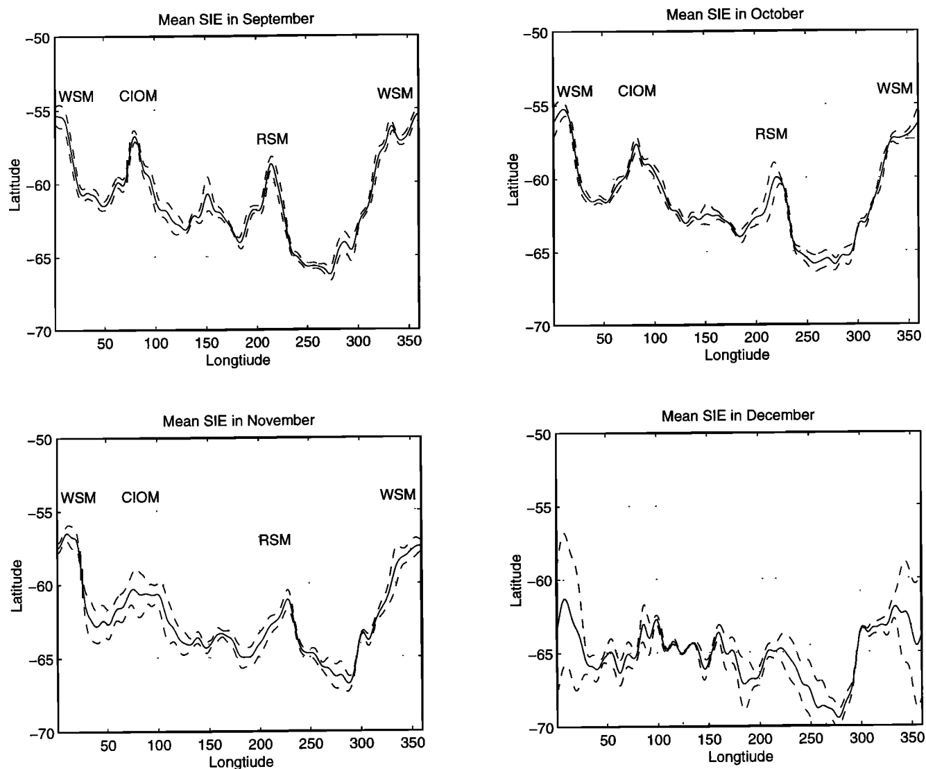
Figure 1. The mean Antarctic sea ice edge (solid lines) derived from Special Sensor Microwave Imager ice concentration data for September, October, November, and December, 1996. Dashed lines indicate one standard deviation. CIOM, RSM, and WSM indicate the central Indian Ocean maximum, Ross Sea maximum, and Weddell Sea maximum, respectively.
