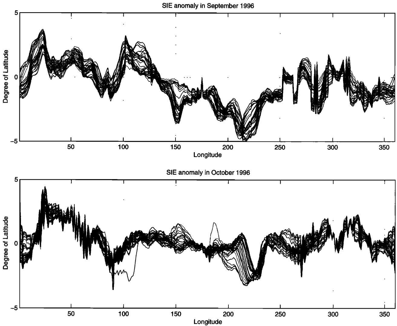
Figure 2. Daily ice edge anomaly in September and October as a function of longitudes.
