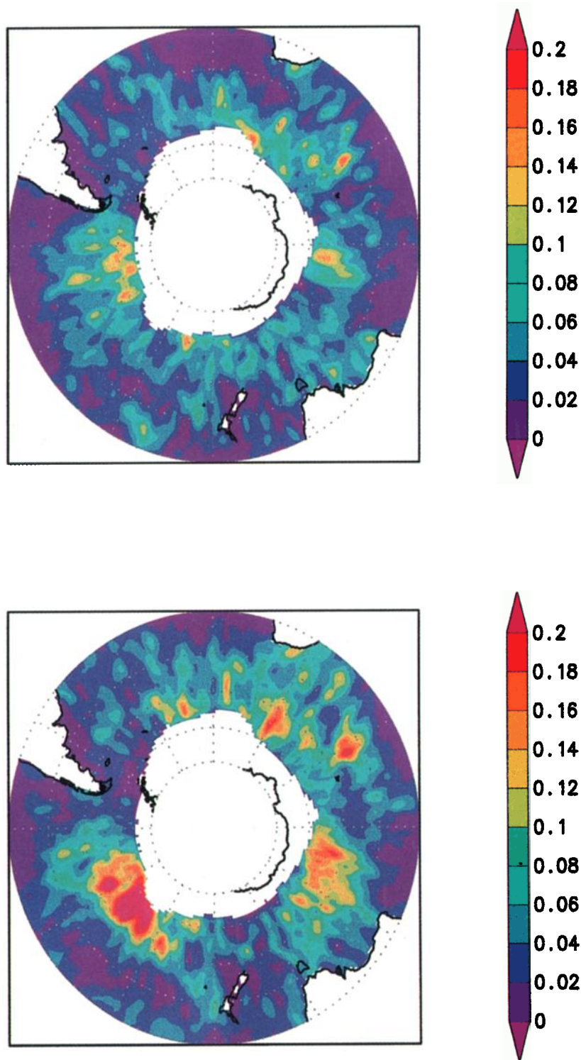
Plate 3. Spectral amplitude for (top) counterclockwise motions and (bottom) clockwise motions in the frequency band of 5-10 days. Twice-daily wind stress data during the maximum ice period (47 days) are used to calculate the spectrum.
