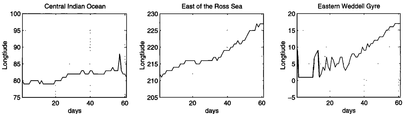
Figure 3. Locations of ice-extent maxima in the central Indian Ocean, east of the Ross Sea, and in the Eastern Weddell Sea as a function of time during September and October, 1996.
