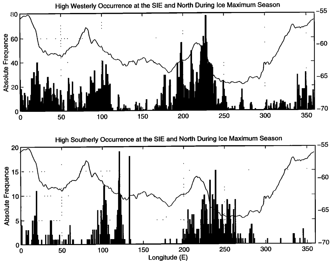
Figure 4. Histograms of high westerlies ( U \geq 10\text{ms}^{-1} ) and high southerlies ( V \geq 10\text{ms}^{-1} ) along the sea ice edge (SIE) as a function of longitude for the ice maximum period. The mean SIE distribution in the same period is superimposed on the histograms.
