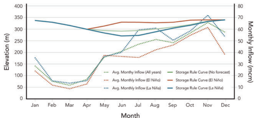
Figure 6.5 Storage rule curves and average monthly inflows to Lake Madden, Panama, for El Niño events, La Niña events and across all years.
