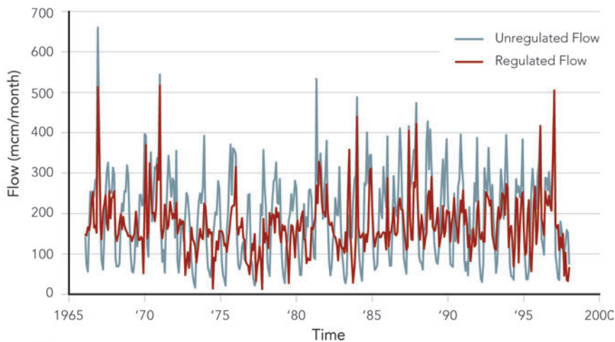
Figure 2.5 Time series of flows on the Chagres River, Panama. Natural (unregulated) flows are shown in blue and regulated flows are shown in red. Regulated flow is generally less variable. Units of flow are million cubic meters (mcm) per month.
