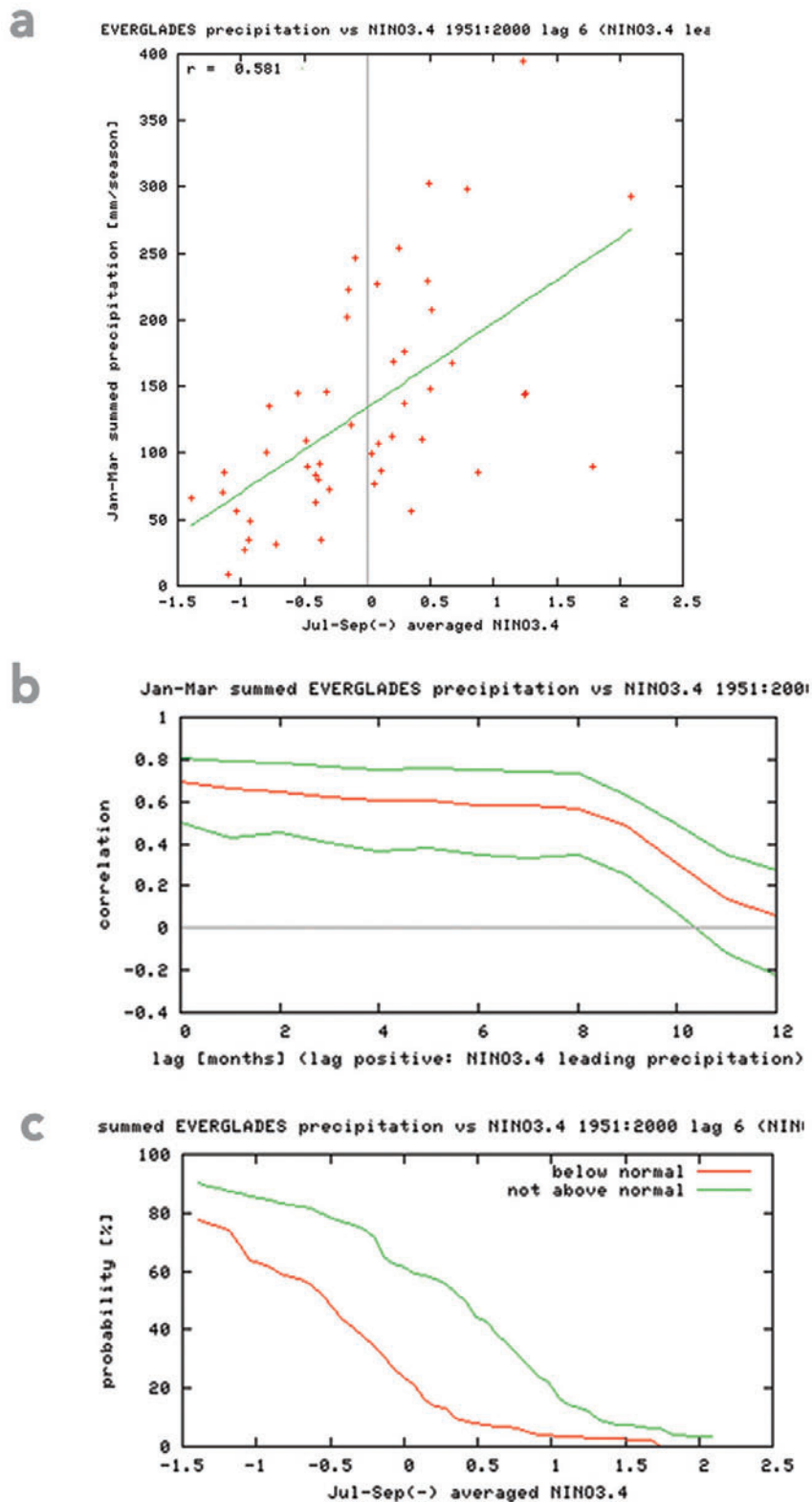
Figure 4.14 Correlation analysis of time series data using the KNMI Climate
