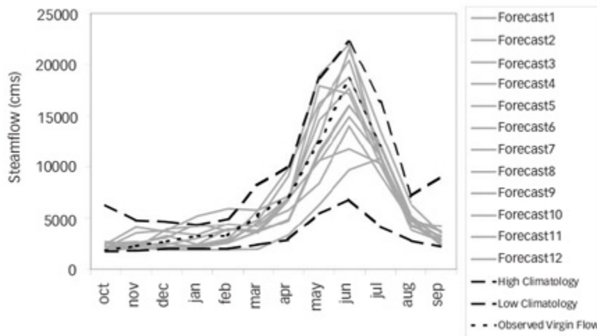
Figure 6.4 Streamflow forecast for the Columbia River for 1999.
