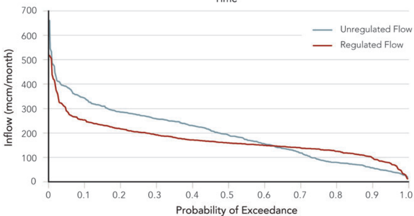
Figure 2.6 Flow-duration curves for flows on the Chagres River, Panama from 1966-1997. Unregulated flows are shown in blue and regulated flows are shown in red. Regulated flows less frequently exceed very high levels or drop below very low levels. Units of flow are million cubic meters (mcm) per month.
