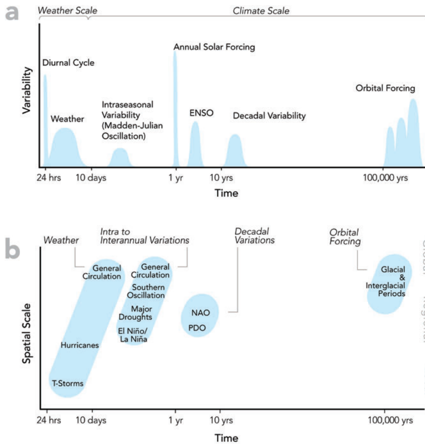
Figure 3.1 Characteristic time and spatial scales of aspects of the climate system.
