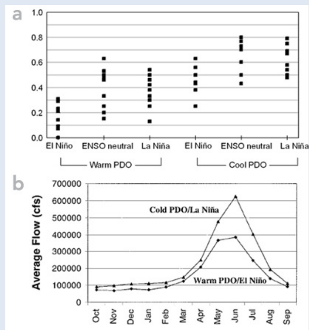
Figure 6.3 Probability of flooding and average historical inflow for the Columbia River based on ENSO and PDO. Panel (a) shows the probability of flooding for snowmelt dominated rivers based on ENSO/PDO phase. A value of .8 is equal to an 80% probability of flooding during spring and summer periods. La Niña conditions and the cool PDO phase increase flooding probability relative to opposite phases. Panel (b) shows the average historical inflow for Columbia River based on ENSO and PDO phase. Units are in cubic feet per second (cfs), where 1 cfs = .0283 cubic meters per second (cms).
