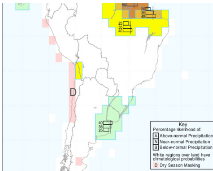
Figure 4.9 An example of a probabilistic seasonal forecast for precipitation made at the IRI. The probabilities on the map represent the relative likelihood of precipitation falling into three tercile categories: Above-Normal, Near-Normal and Below-Normal. These three categories are determined by ranking the seasonal precipitation over the 30-year period 1971-2000.
