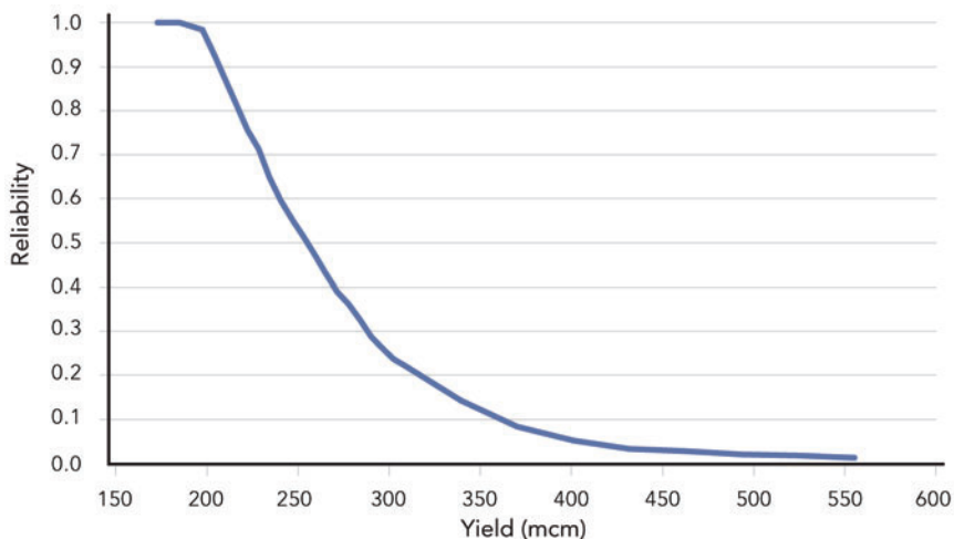
Figure 2.10 Yield-reliability relationship based on the standard operating policy (SOP). Reliability represents the fraction of months during which the supply target is met. A value of .8 means it was met 80% of the time.
