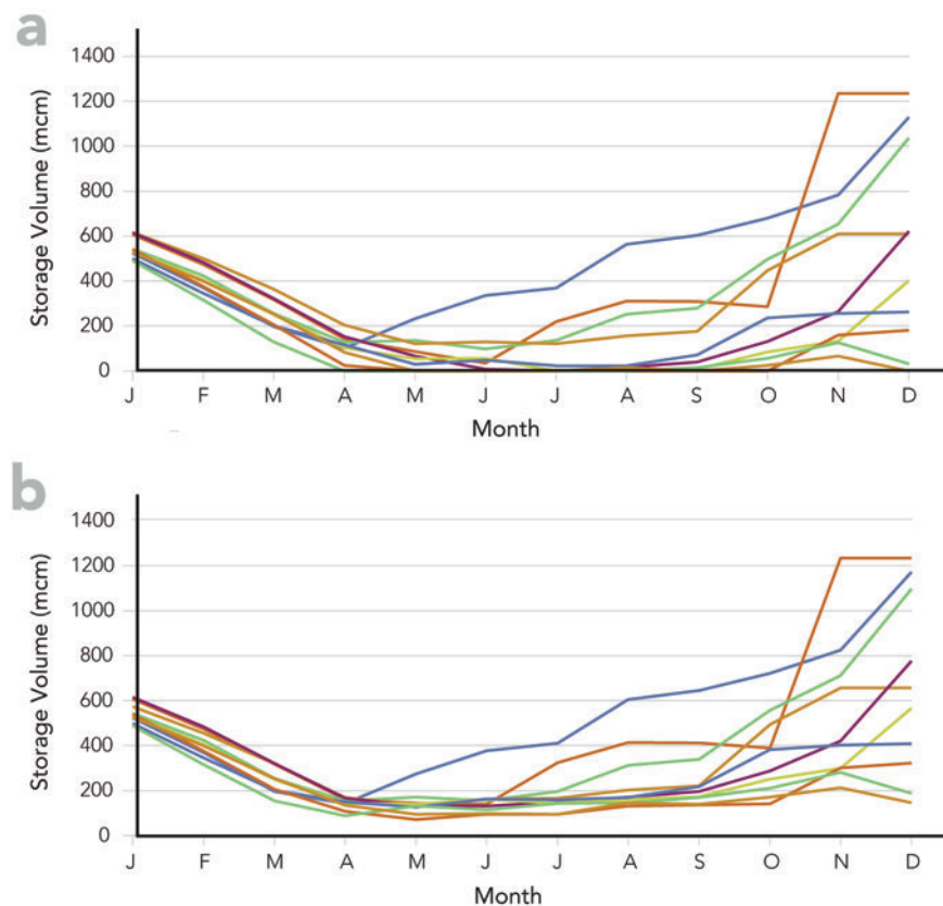
Figure 2.12 Position analysis based on historical inflow traces. Panel (a) shows traces using the standard operating policy (SOP), and Panel (b) shows traces using the hedging policy. Each trace represents the storage volume based on the given operating policy and inflow from a specific year in the historical record. The hedging policy prevents the storage volume from dropping below a threshold level of around 100mcm.
