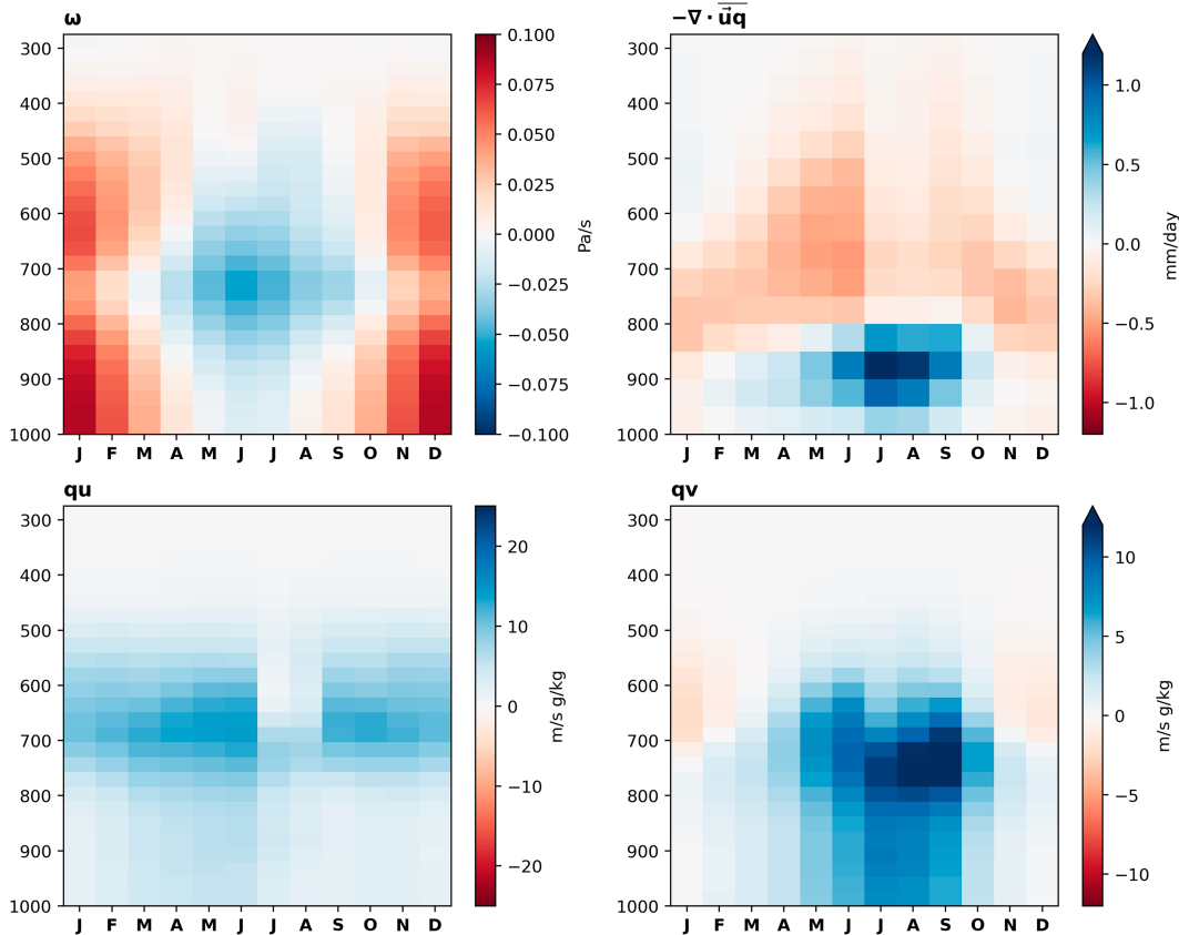
FIG. 6. (top left) Monthly climatology of subsidence ( \omega ), (top right) horizontal moisture convergence by the mean flow ( -\nabla \cdot \bar{q}\bar{u} ), (bottom left) zonal moisture transport ( qu ), and (bottom right) meridional moisture transport ( qv ) at pressure levels from 1000 to 250 hPa, in the 32^{\circ} – 37^{\circ} N, 104^{\circ} – 114^{\circ} W region over the 1970–2019 period.
