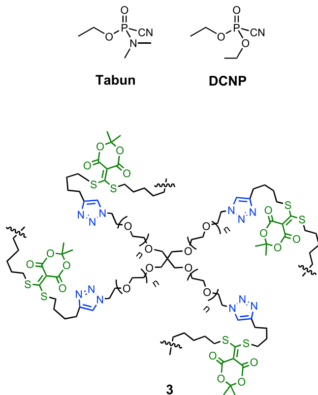
Scheme 2. Selected tabun surrogate and synthesized hydrogel
