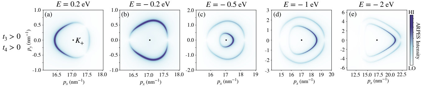
FIG. 11. Constant-energy ARPES momentum distributions, using y -polarized light, near \mathbf{K}_+ at various energies. The tight-binding parameters are the same as in Fig. 9(1a-1e). Note that we use a power-law normalized colorbar.
