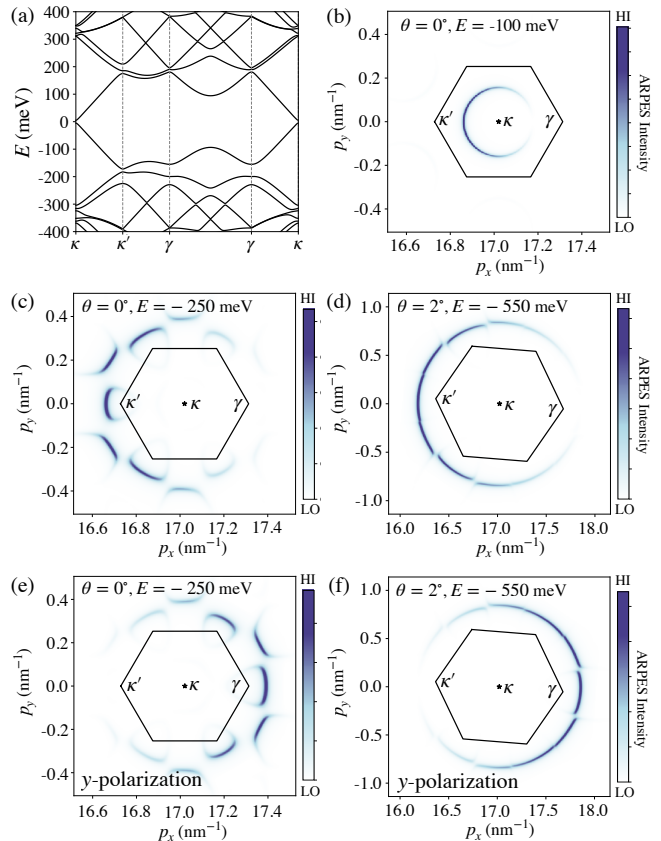
FIG. 1. (a) Moiré band structure of G/hBN with twist angle \theta = 0^\circ , calculated using the ab initio relaxed first harmonic parameters from Ref.58. (b-d) Constant-energy ARPES momentum distributions near BZ corner \mathbf{K}_+ calculated using Eq. (3) in which a factor related to photon polarization is dropped. (b) \theta = 0^\circ at energy E = -100 meV, where hBN substrate has little effect on the energy bands; (c) \theta = 0^\circ at energy E = -250 meV, where the hBN substrate has a large effect on the energy bands of graphene; (d) \theta = 2^\circ at E = -550 meV. hBN's effect is negligible when the graphene and hBN layers are away from alignment. (e-f) Constant-energy ARPES momentum distributions calculated for y -polarized light using Eq. (4). The x -polarized light yields ARPES contours identical to those calculated in (c-d) using Eq. (3). Photons with y -polarization rotate the anisotropy by \pi compared to photons with x -polarization. In (b-f), the hexagon is the MBZ.
