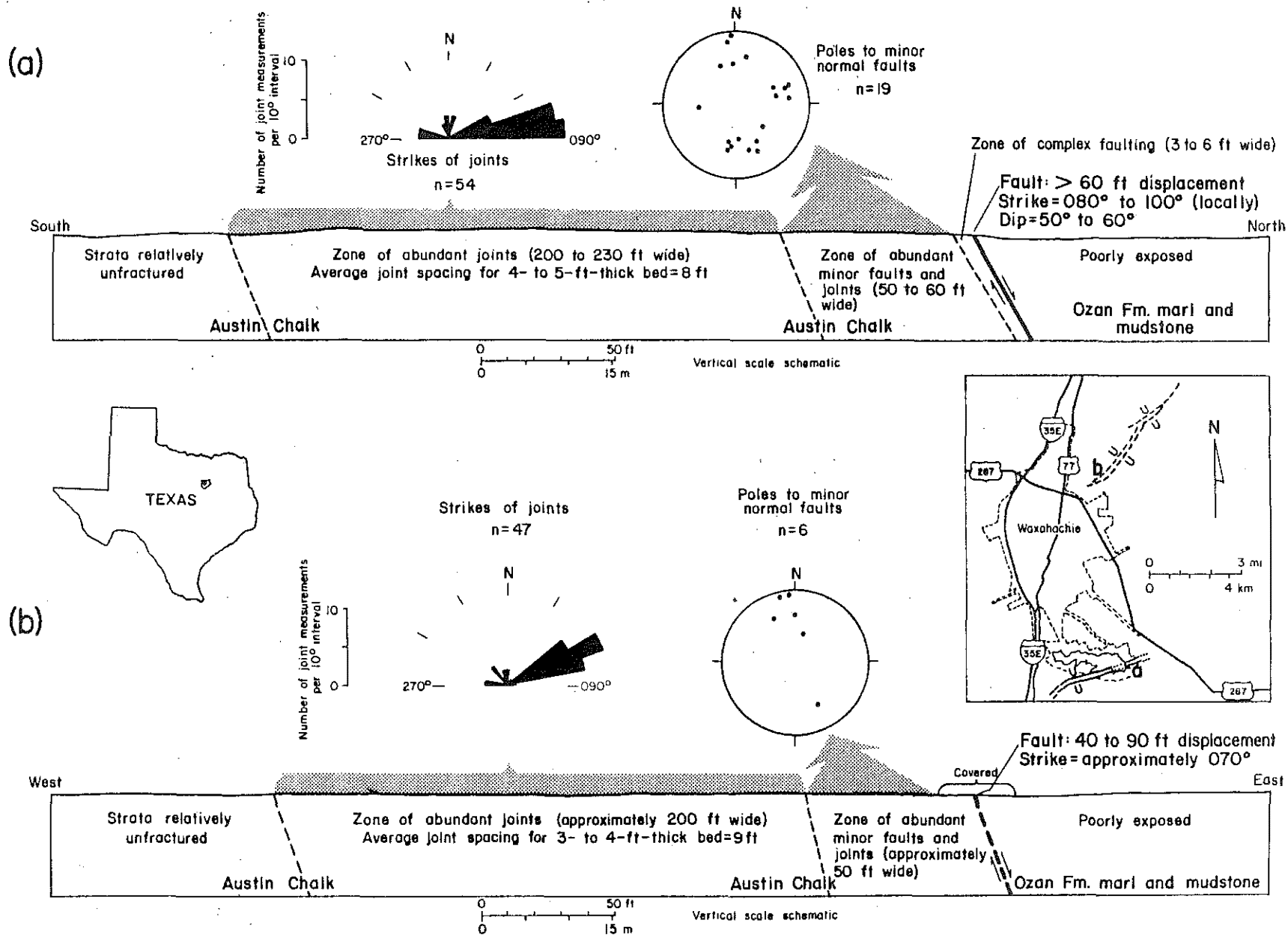
Figure 3. Fracture styles, geometries, and intensities of adjacent major normal faults at (a) graben near Lake Waxahachie and (b) graben northeast of Waxahachie.
