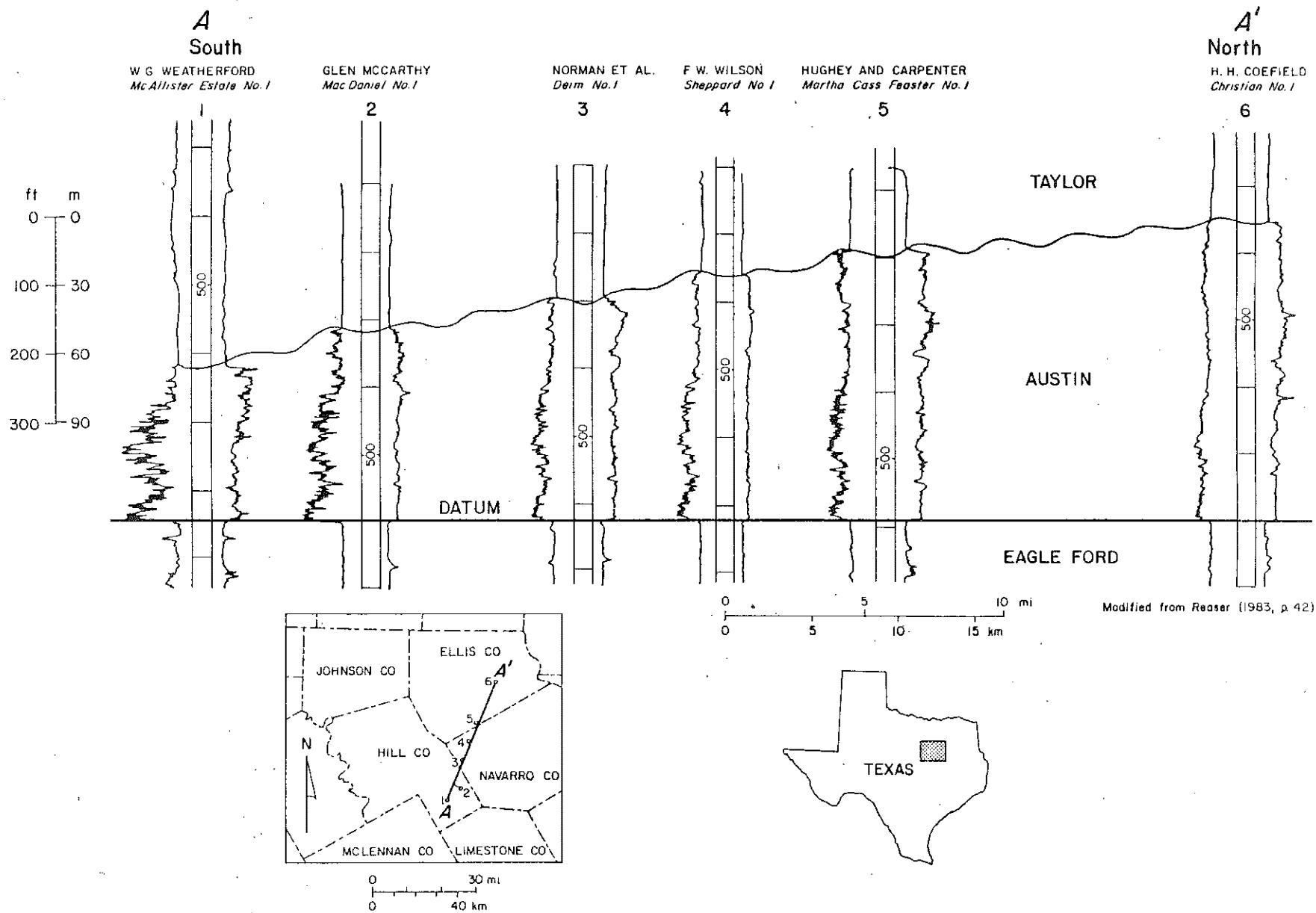
Figure 2. Stratigraphic section of upper Eagle Ford, Austin, and lower Taylor in Ellis, Hill, and Navarro Counties, Texas. Vertical scale: 1 inch = 100 ft.
