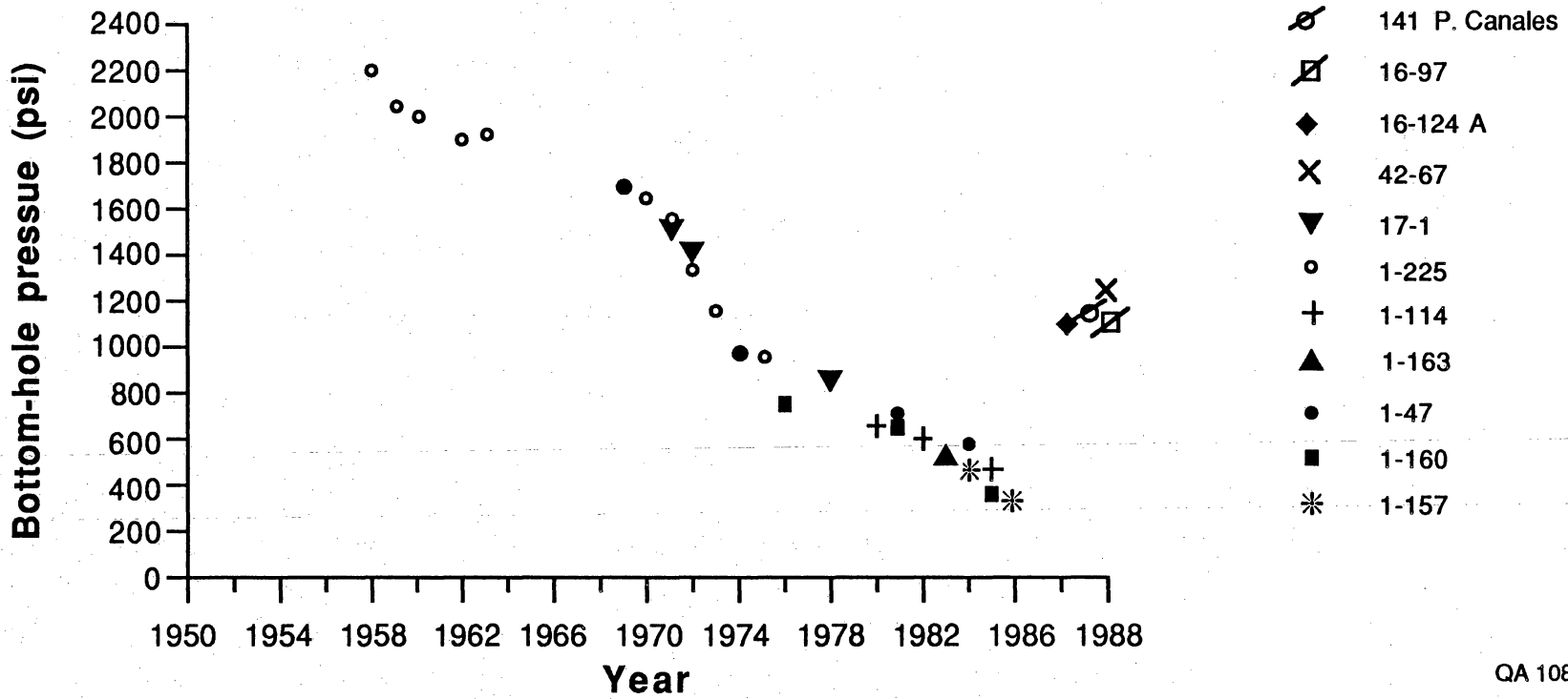
Figure 38. Bottom-hole pressure versus time for 11 wells productive in Zone 15 (data from Sun Exploration and Production, Inc.).
