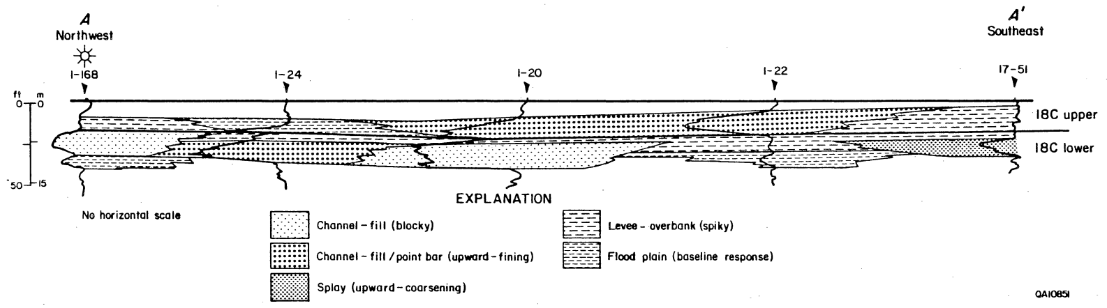
Figure 45. Stratigraphic cross section A-A' illustrating upper and lower sandstones within Zone 18-C (see fig. 46 for location). Recompletion target is channel-fill/point-bar sandstone of 18-C upper in well 1-22. Facies changes in both upper and lower units should compartmentalize 18-C lower reservoir in well 1-168 and isolate potential gas-bearing 18-C upper zone in well 1-22.
