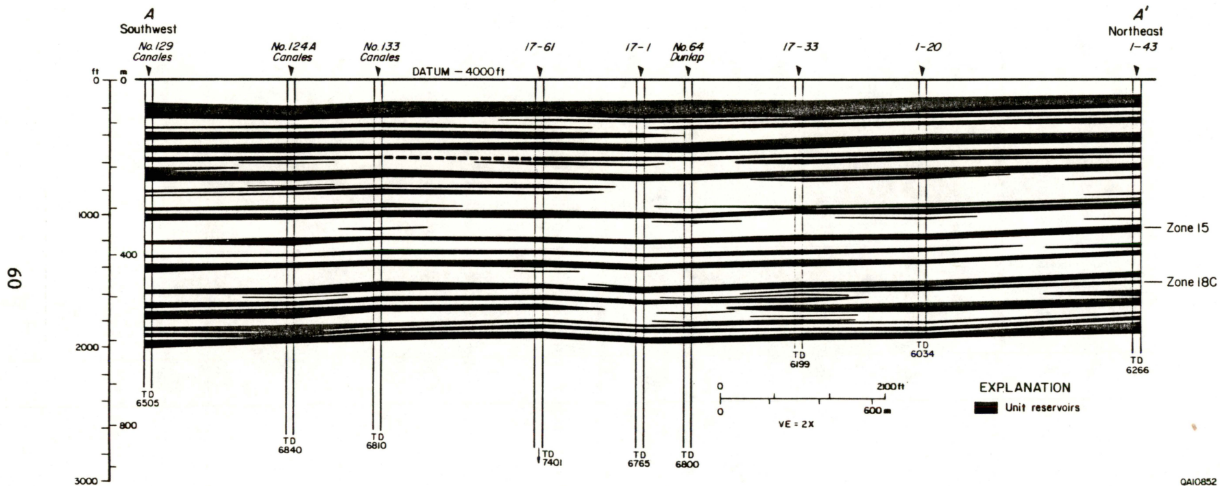
Figure 26. Schematic structural strike-section A-A' through east-central part of Seeligson field (see fig. 25 for location). Multiple, vertically stacked, multilateral reservoirs are characteristic of the field. Zones 15 and 18-C were studied in detail.
