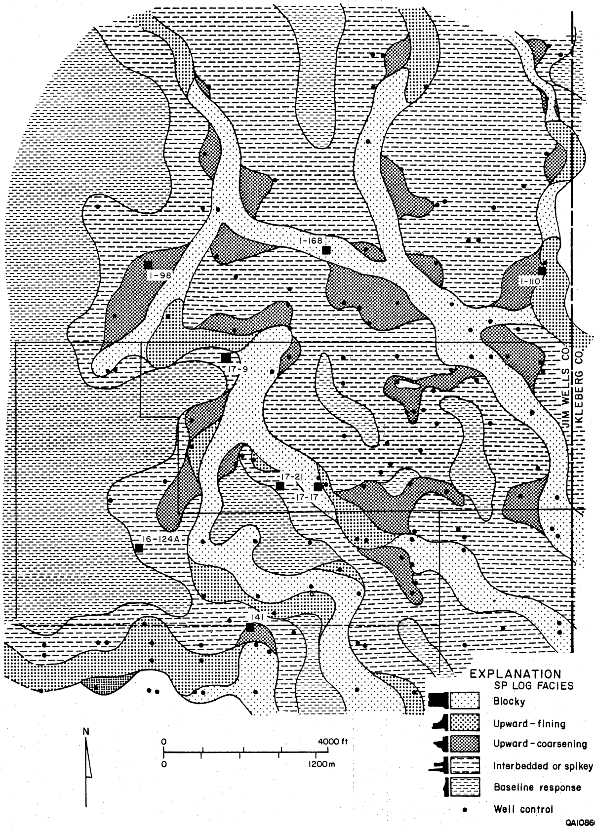
Figure 43. SP log facies map of Zone 15-C. Crevasse splay deposits are more widespread than in Zone 15-B. Localized muddy areas may represent mud plugs in abandoned channels.
