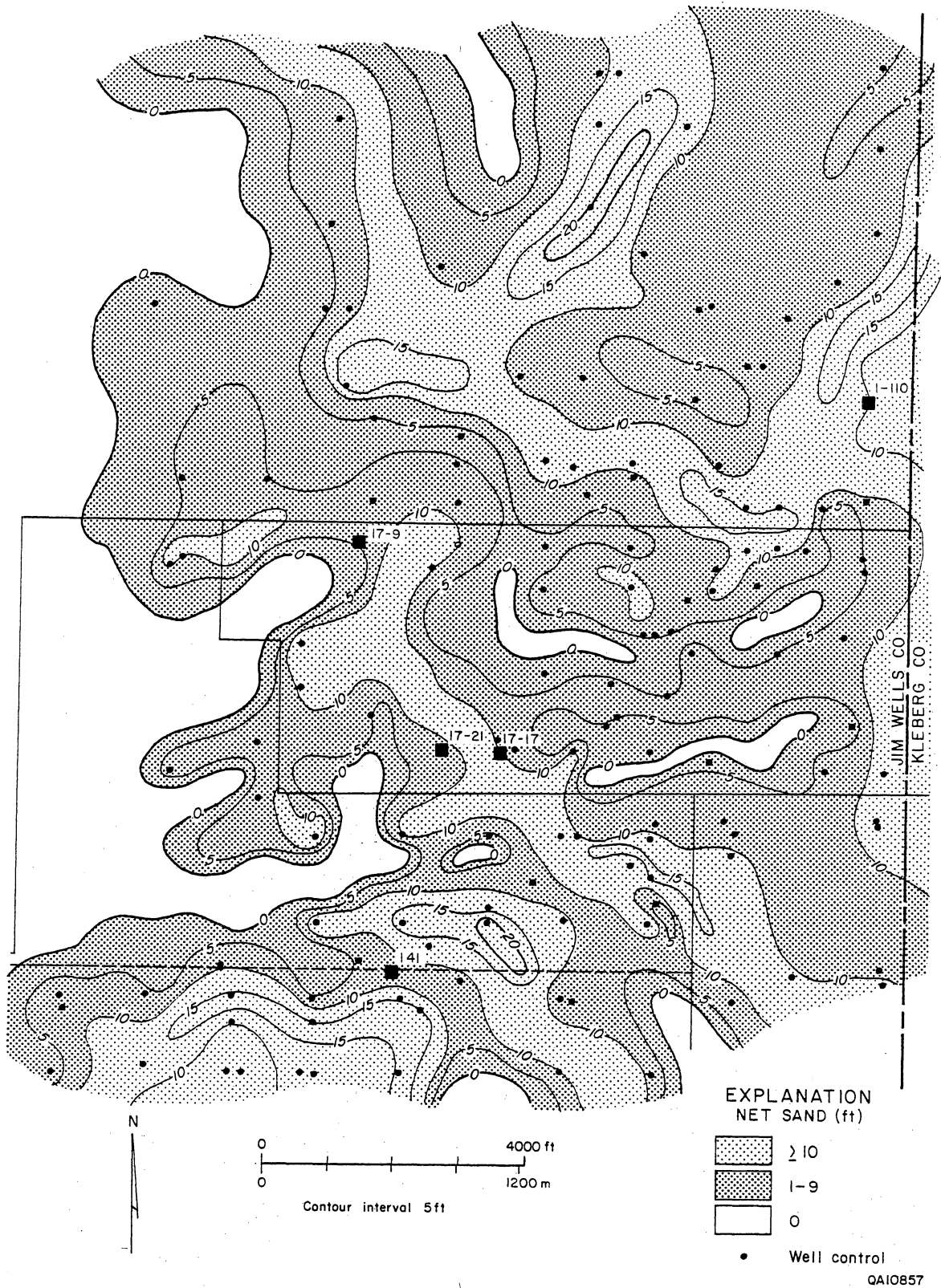
Figure 42. Net-sandstone isopach of Zone 15-C. Primary depositional axes occur in the northeastern, central, and southwestern parts of the area. Sandstones pinch out in several localized areas and near the western edge of the study area.
