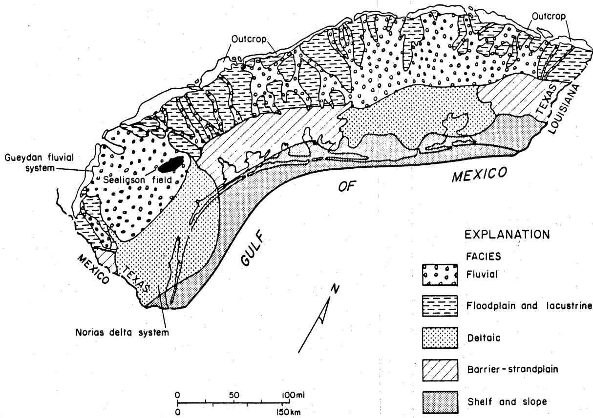
Figure 27. Frio depositional systems along the Texas Gulf Coast. Middle and upper Frio sediments were deposited in the Gueydan fluvial system, which consisted of a network of low-sinuosity bed-load streams in the Rio Grande Embayment (modified from Galloway and others, 1982).
