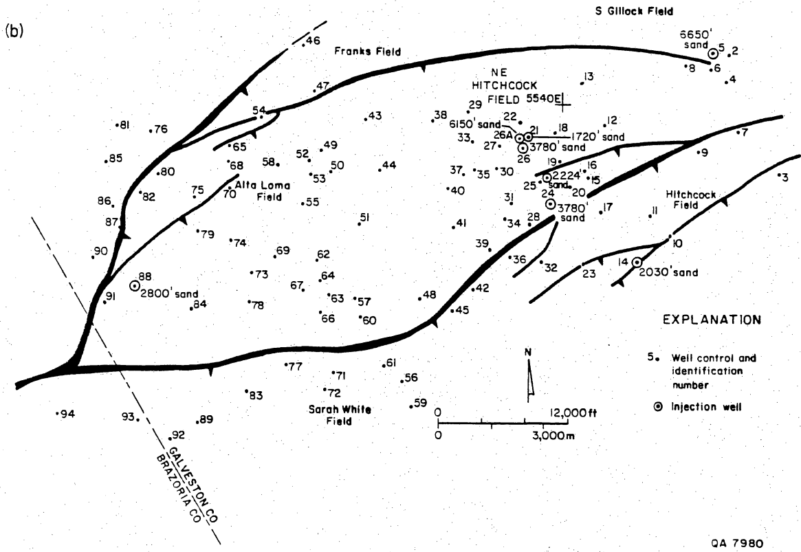
Figure 10. (a) Structure map of Northeast Hitchcock and Alta Loma fields, contoured on top of the 4,240-ft sand (middle Miocene). Two major growth faults, with throws from 50 to 200 ft, isolate these two fields into a 35-mi 2 fault block. (b) Well control used in this study. Miocene sands in six of these wells have received brines; these wells and sands are indicated on the map above. Amounts of disposed brine are indicated on net-sand maps.
