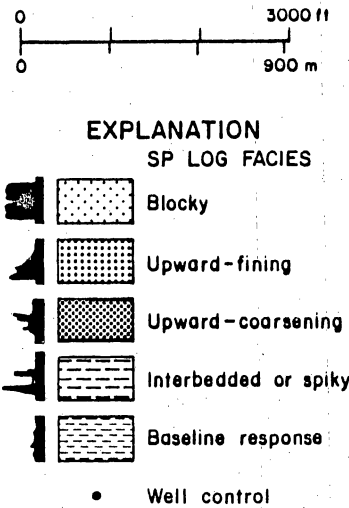
Figure 32. SP log facies of Zone 11-B. Blocky and upward-fining log curve shapes define reservoir-quality channel-fill deposits. Upward-coarsening patterns represent crevasse splay sands; spiky and baseline log responses are indicative of levee-overbank and floodplain facies.
