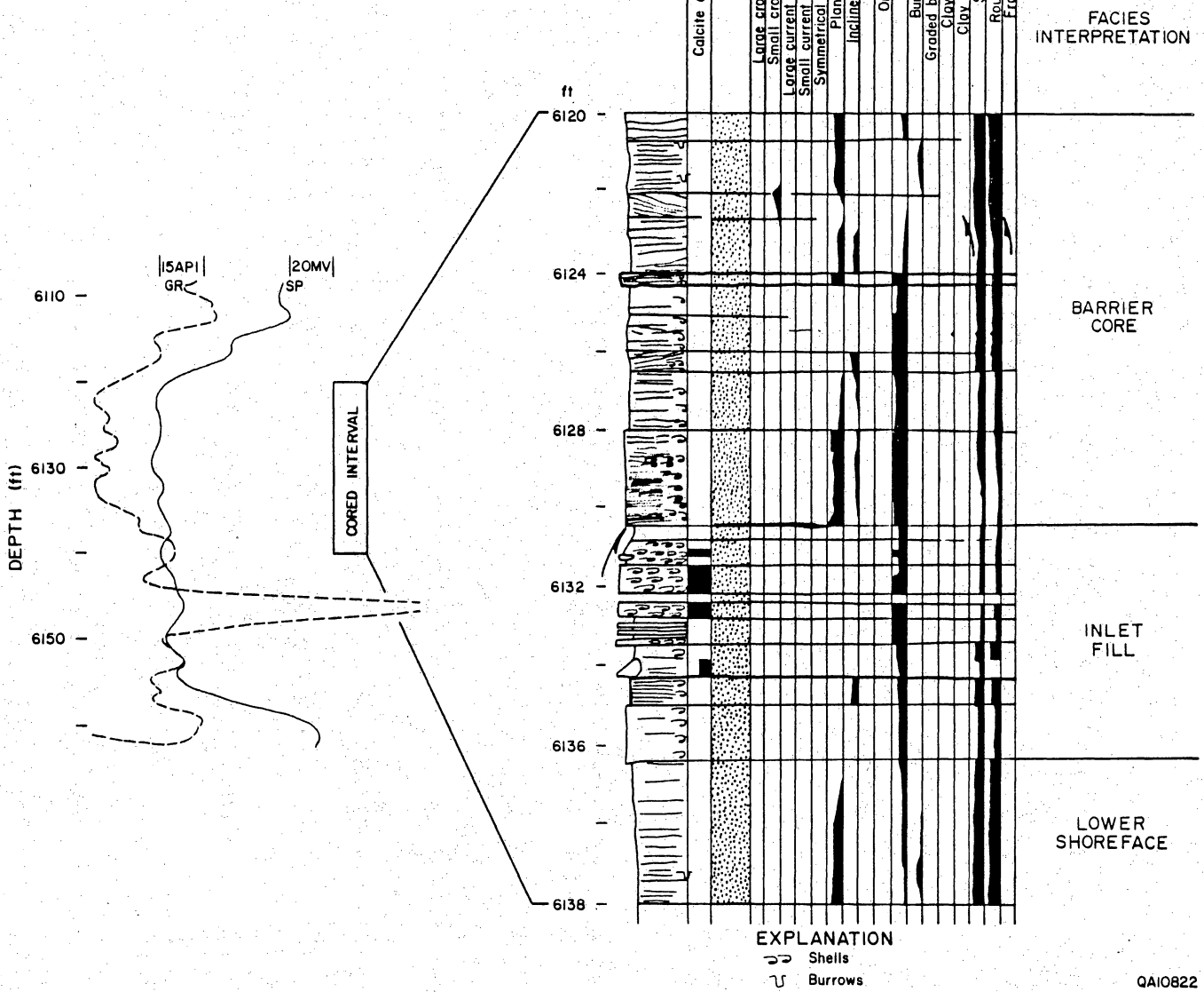
Figure 21. Core description and log response of the 6,150-ft sand (lower Miocene) from the H. D. S. Thompson No. 3 brine-disposal well in Northeast Hitchcock field.
