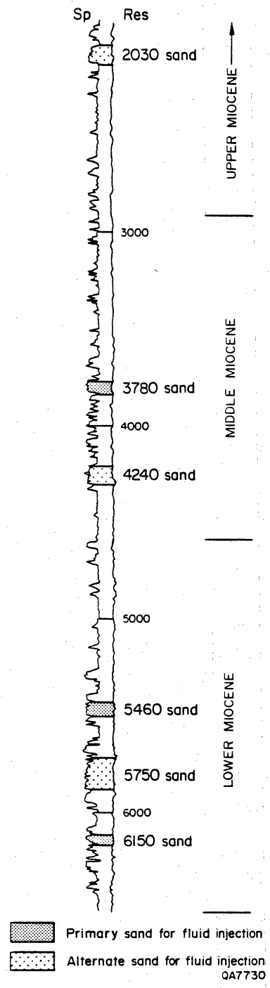
Figure 12. Type log (Phillips Thompson No. 1; number 26 in this study) in Northeast Hitchcock field. The three best zones for brine disposal (3,780 ft, 5,460 ft, and 6,150 ft) are in barrier-island depositional units that contain large volumes of homogeneous barrier-core facies. Three alternate sands (2,030 ft, 4,240 ft, and 5,750 ft) are also shown.
