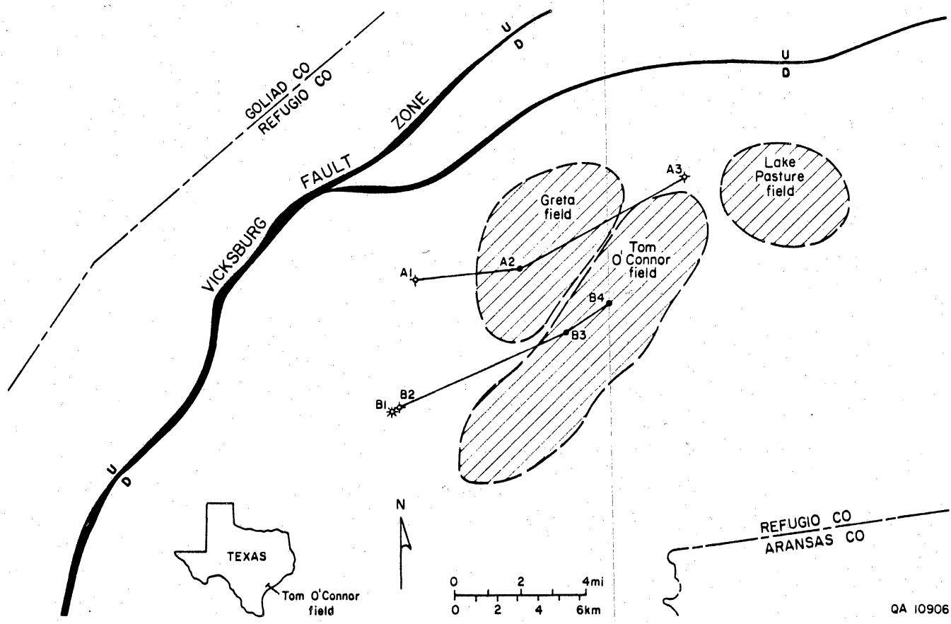
Figure 51. Index map. Location of Tom O'Connor field is shown along with that of adjacent fields with production from Miocene sandstones. Growth faults in the Vicksburg Fault Zone were apparently active during deposition of lower Miocene sediment. Cross sections A and B are illustrated in figure 52.
