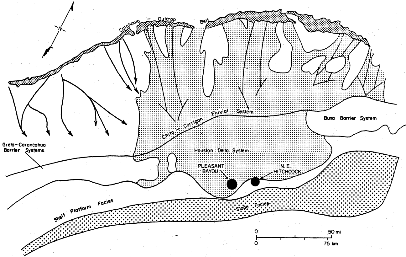
Figure 2. Regional depositional setting of Northeast Hitchcock field, Galveston County, and Pleasant Bayou geopressedured-geothermal test wells, Brazoria County, Texas (modified from Galloway and others, 1982).
