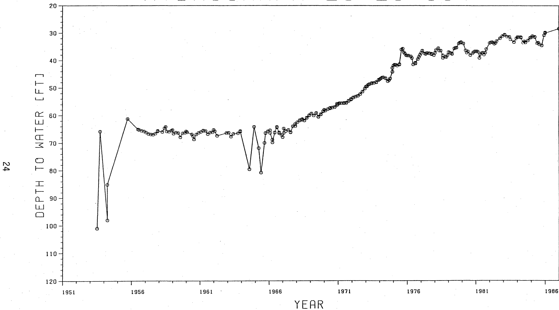
Figure 13. Water-level hydrograph of well 23-25-304. Water-level data from Texas Natural Resources Information System. Location of well shown in Figure 6.
