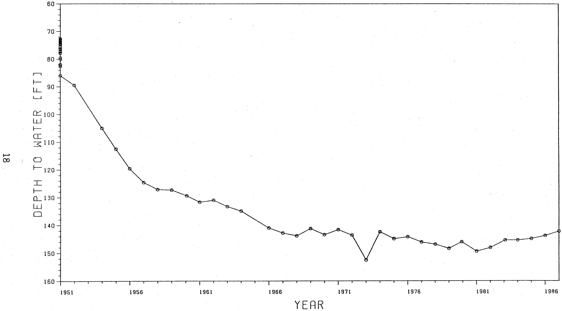
Figure 8. Water-level hydrograph of well 23-25-401. Water-level data from Texas Natural Resources Information System. Location of well shown in Figure 6.
