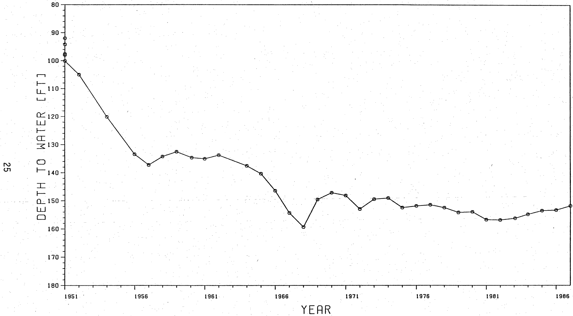
Figure 14. Water-level hydrograph of well 23-34-903. Water-level data from Texas Natural Resources Information System. Location of well shown in Figure 6.
