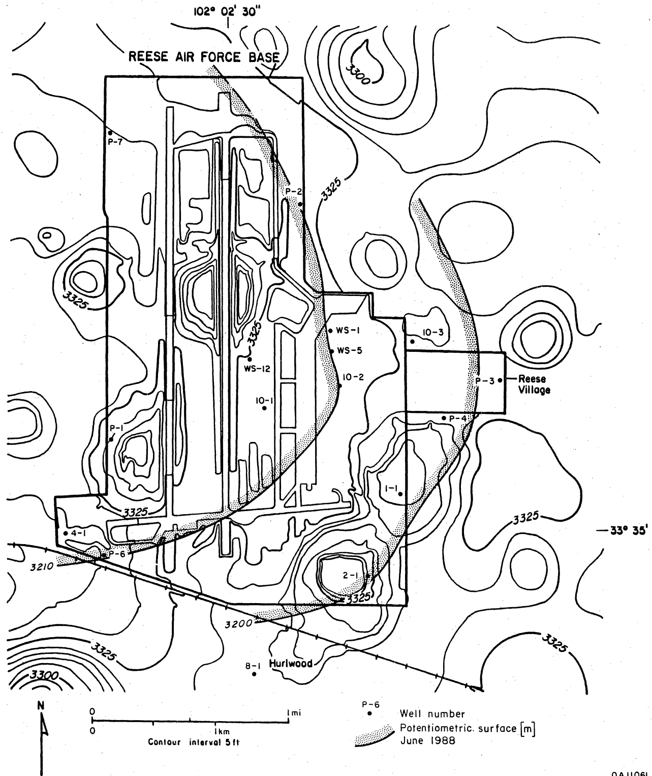
Figure 23. Local potentiometric surface, water levels from June 1988.
