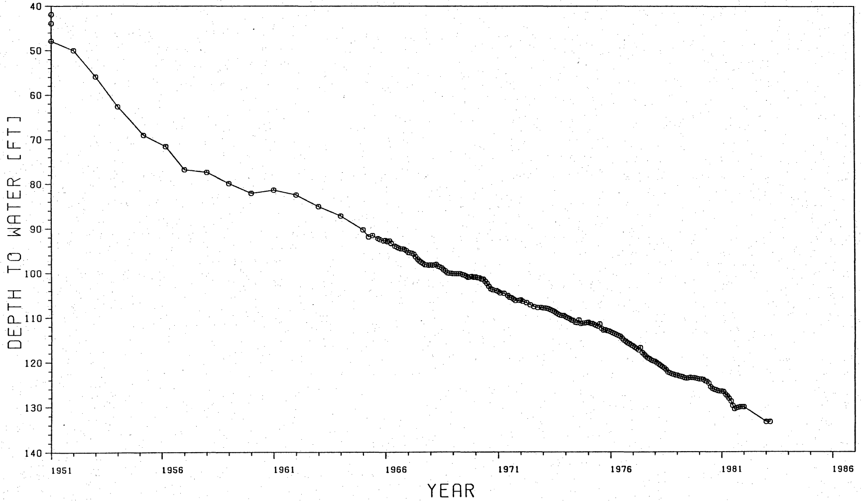
Figure 15. Water-level hydrograph of well 11-51-503. Water-level data from Texas Natural Resources Information System. Location of well shown in Figure 6.
