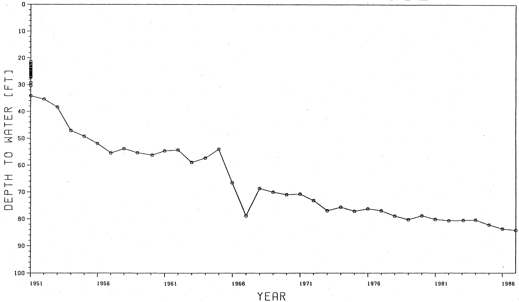
Figure 12. Water-level hydrograph of well 23-17-802. Water-level data from Texas Natural Resources Information System. Location of well shown in Figure 6.
