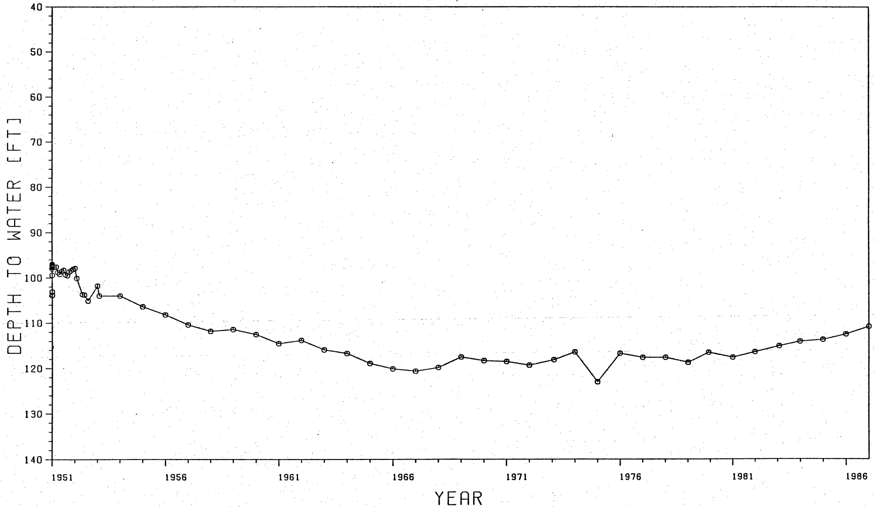
Figure 16. Water-level hydrograph of well 24-31-601. Water-level data from Texas Natural Resources Information System. Location of well shown in Figure 6.
