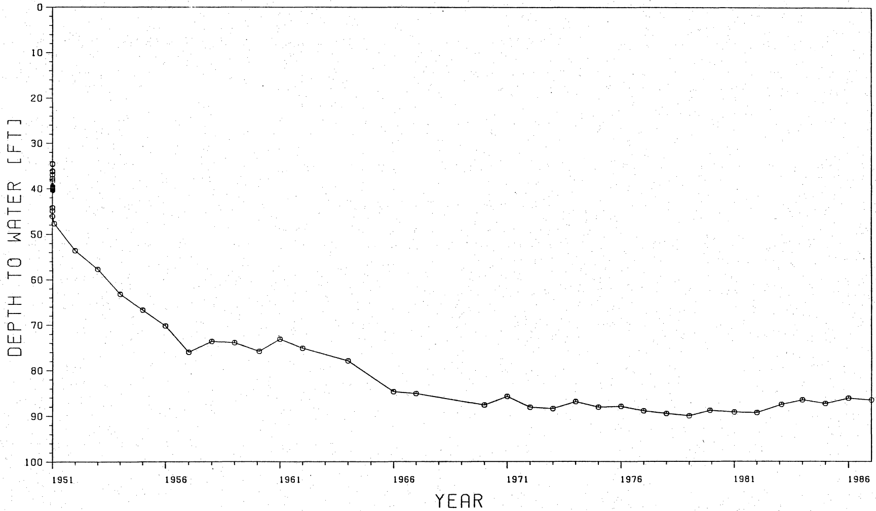
Figure 11. Water-level hydrograph of well 23-17-801. Water-level data from Texas Natural Resources Information System. Location of well shown in Figure 6.
