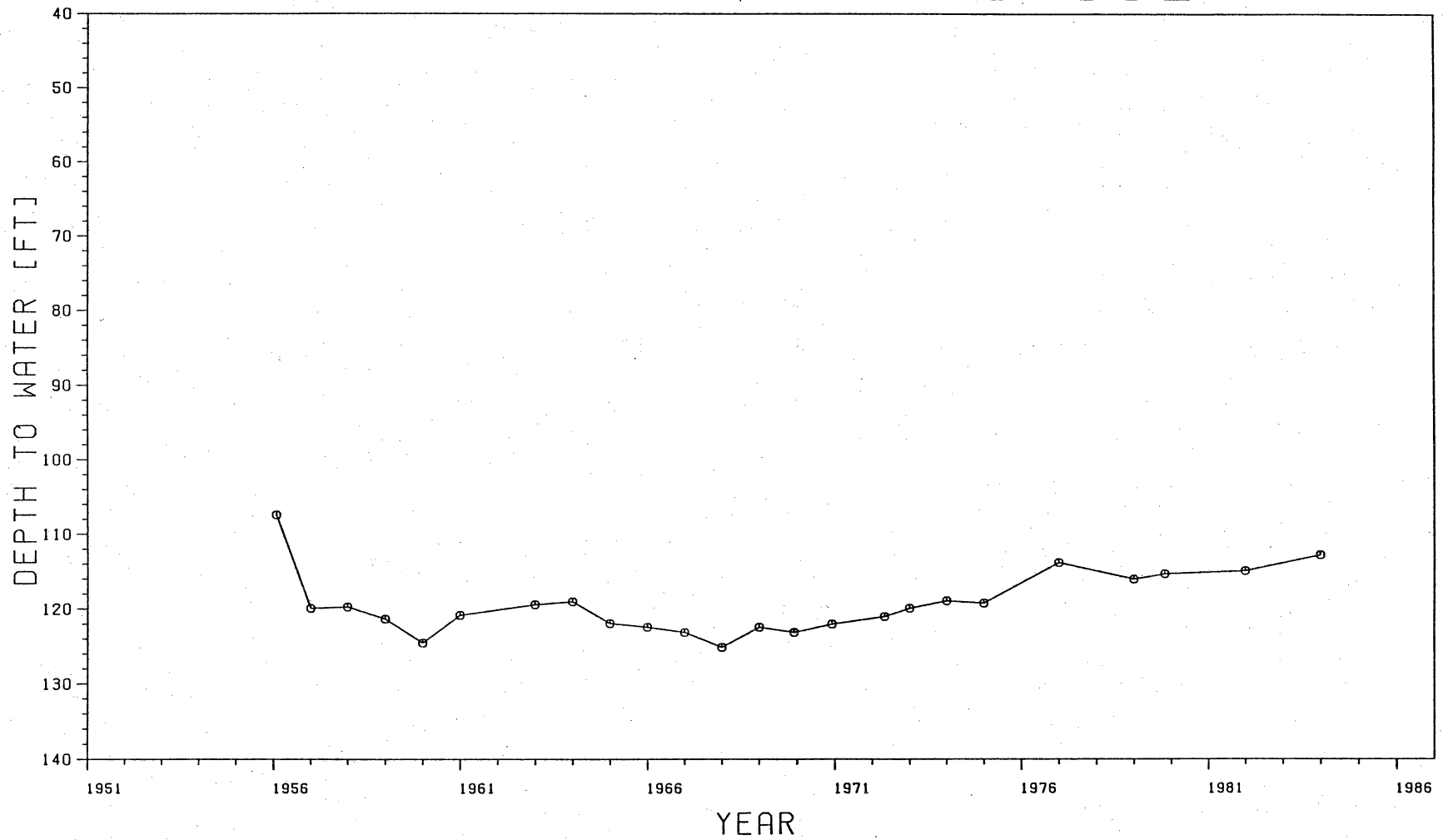
Figure 17. Water-level hydrograph of well 24-45-902. Water-level data from Texas Natural Resources Information System. Location of well shown in Figure 6.
