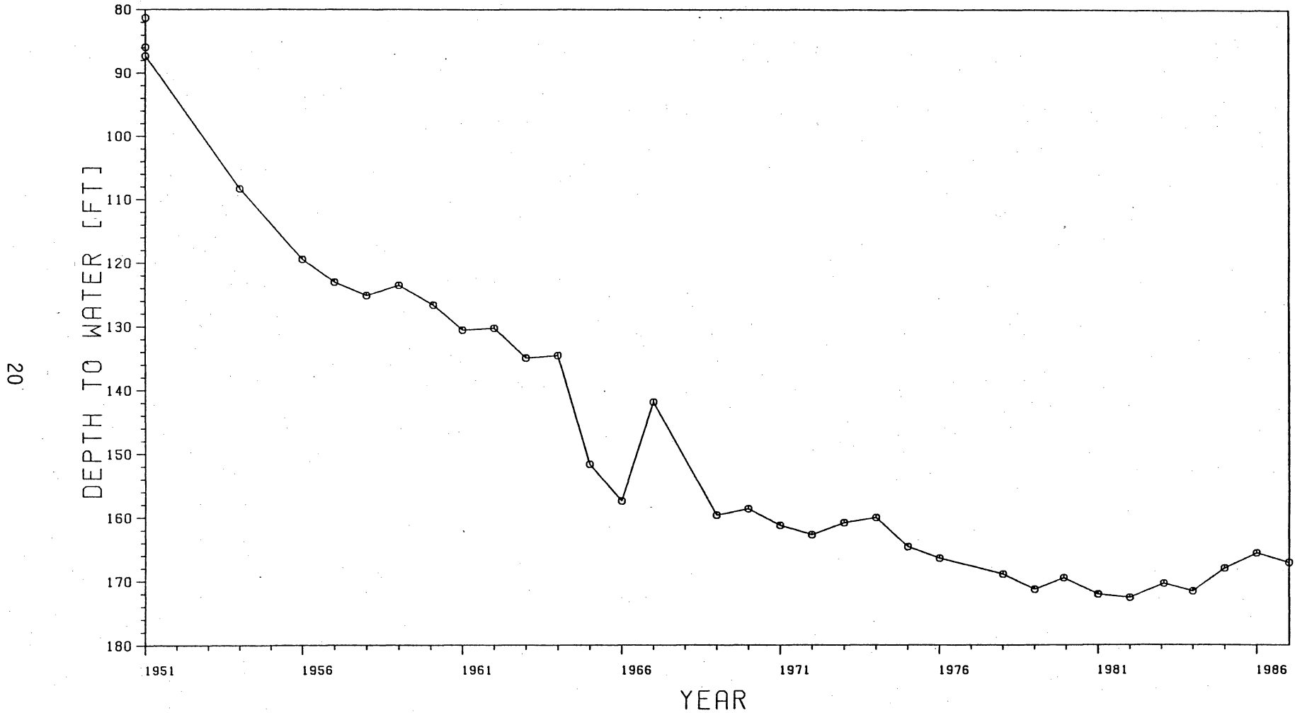
Figure 10. Water-level hydrograph of well 24-24-901. Water-level data from Texas Natural Resources Information System. Location of well shown in Figure 6.
