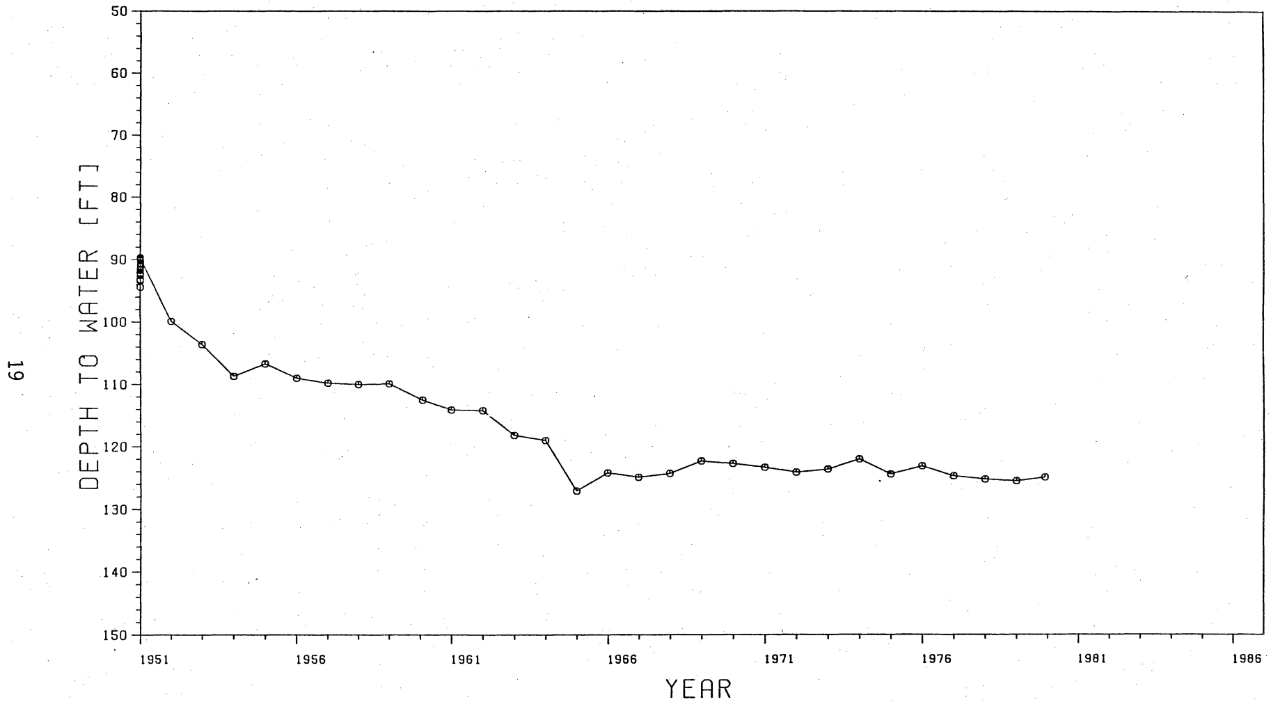
Figure 9. Water-level hydrograph of well 24-32-501. Water-level data from Texas Natural Resources Information System. Location of well shown in Figure 6.
