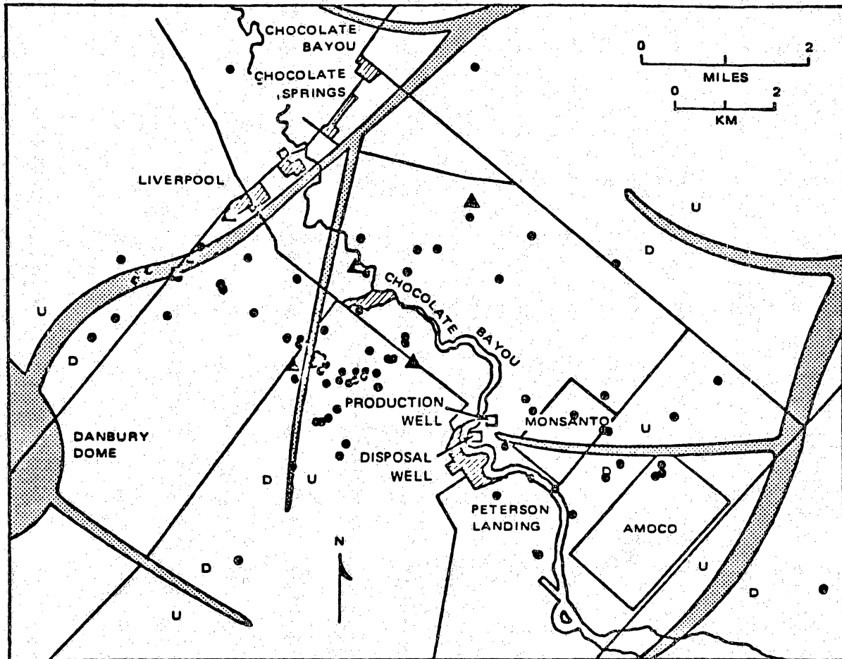
▲ STATIONS ● NATURAL EVENTS * HIGH-RATE SEQUENCE ■ PUMP NOISE Figure 17. Cumulative epicenter map for natural events as of May 30, 1980.
