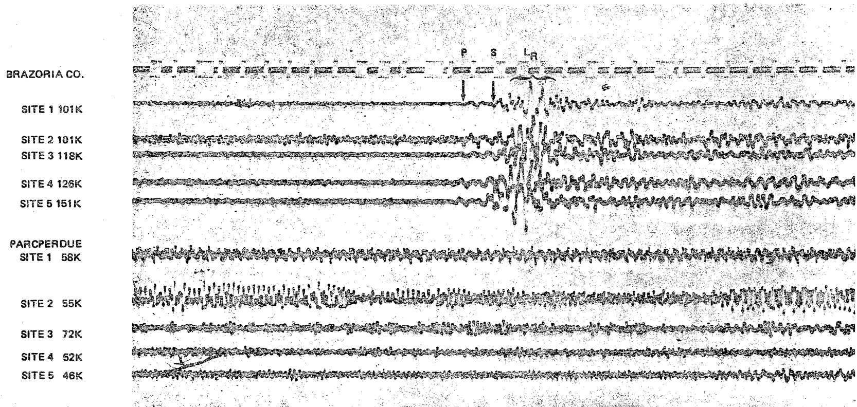
Figure 8. Background noise samples with microseismic event (magnitude 1.6), 1 January 1981 03:32:29.29 UCT (31 December 1980 21:32:29.29 CST).
