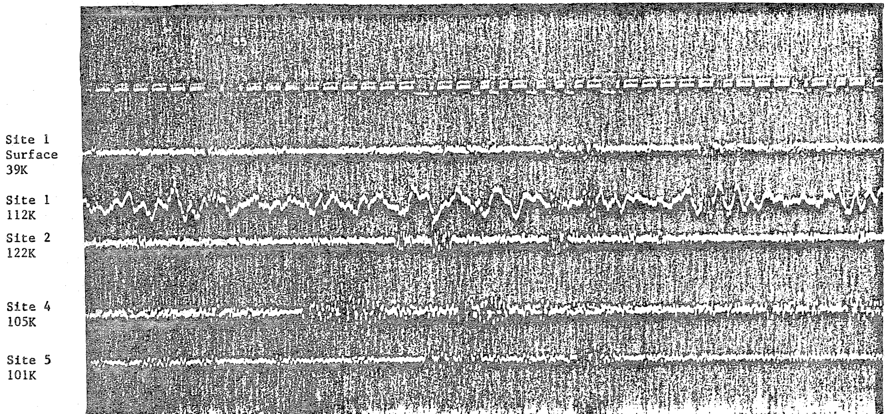
Figure 11. Typical record from night of February 5-6.
