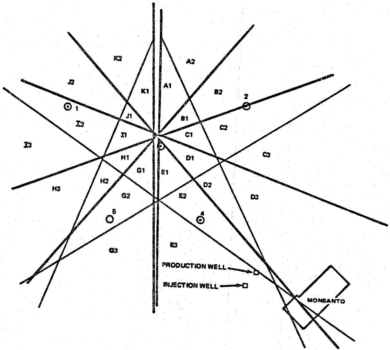
Figure 13. Epicentral regions and station locations.
