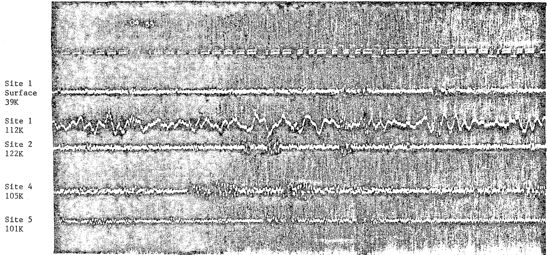
Figure 6. Typical surface wave event, February 5 and 6, 1980.
