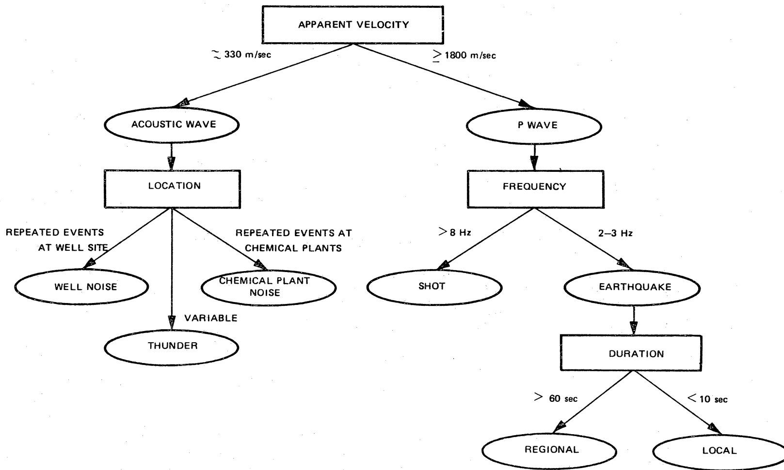
Figure 4. Tentative classification of events by source type.
