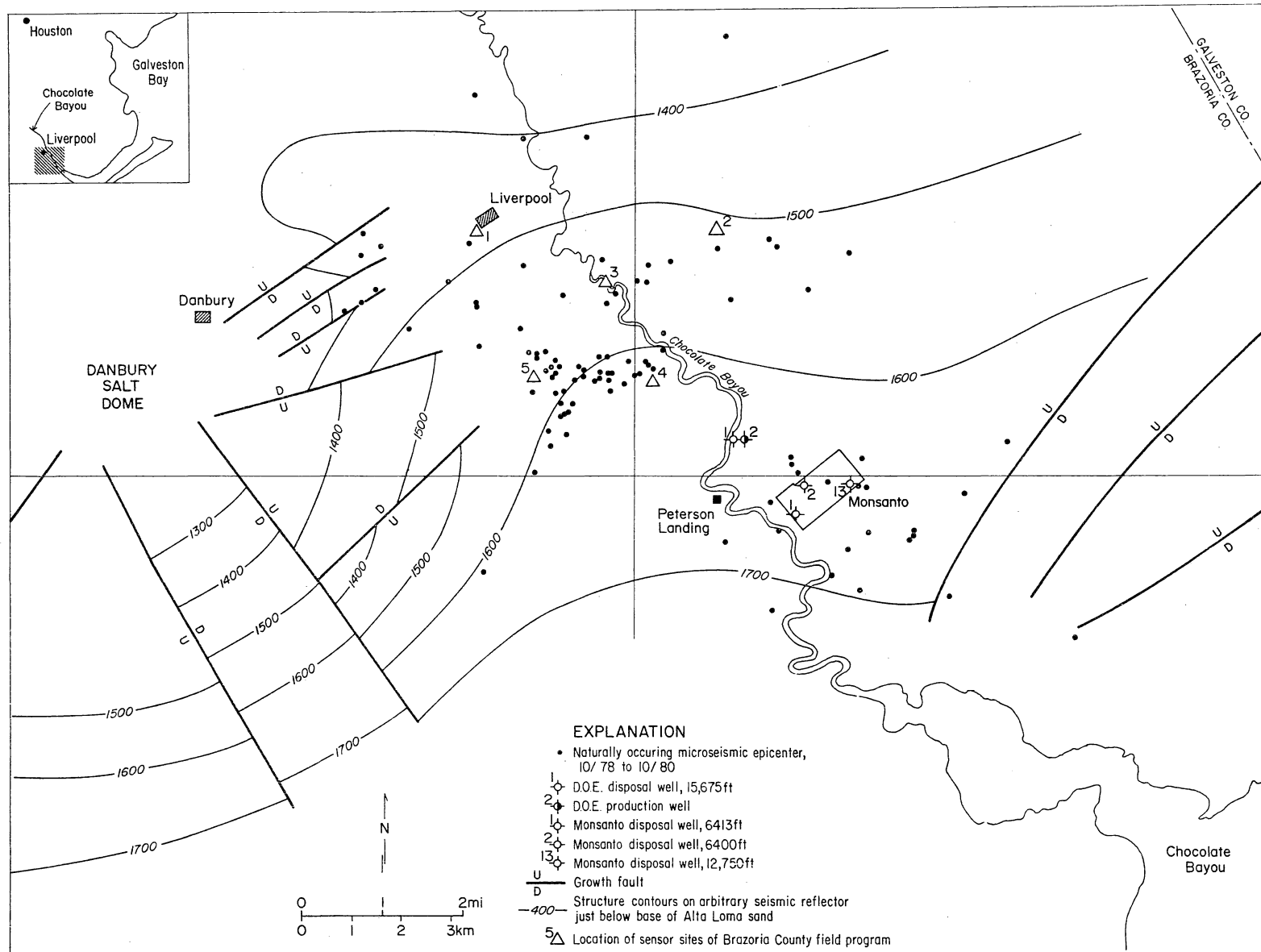
Figure 8. Structure contours on arbitrary seismic reflector just below base of Alta Loma sand and cumulative epicenter map for natural events as of October 31, 1980.
