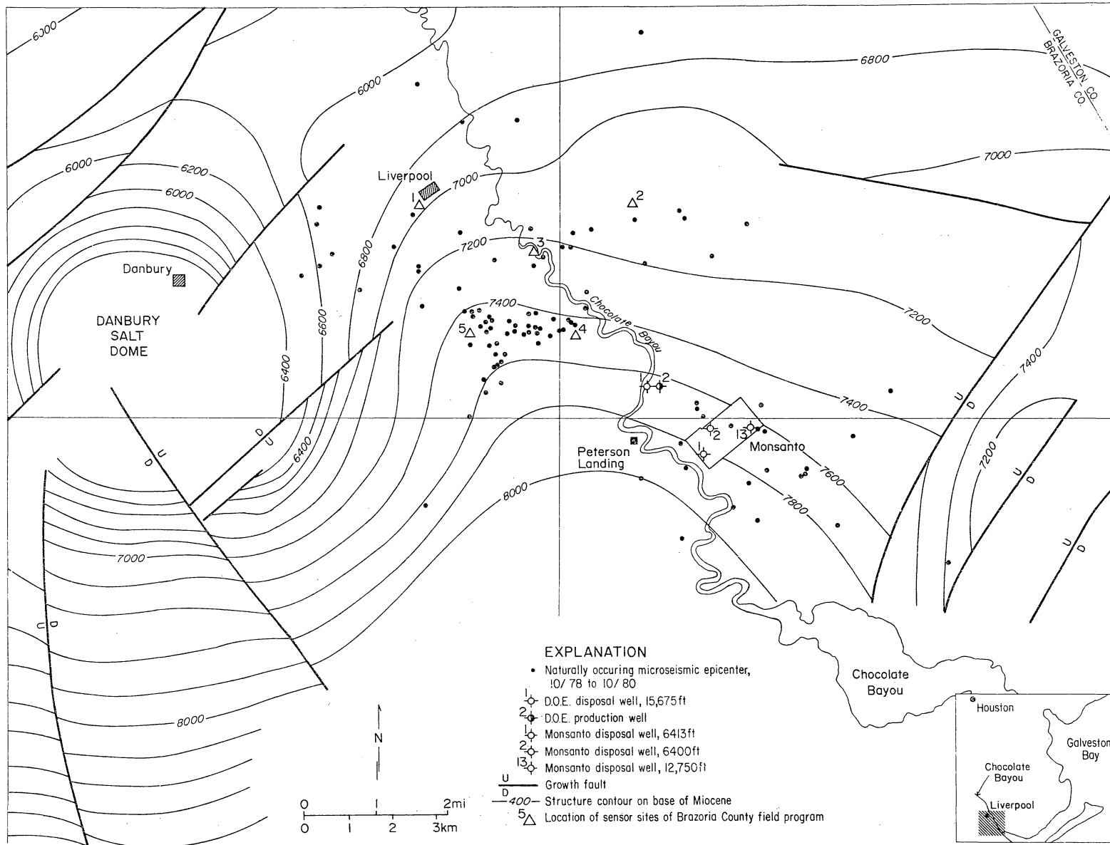
Figure 7. Structure contours on base of Miocene and cumulative epicenter map for natural events as of October 31, 1980.
