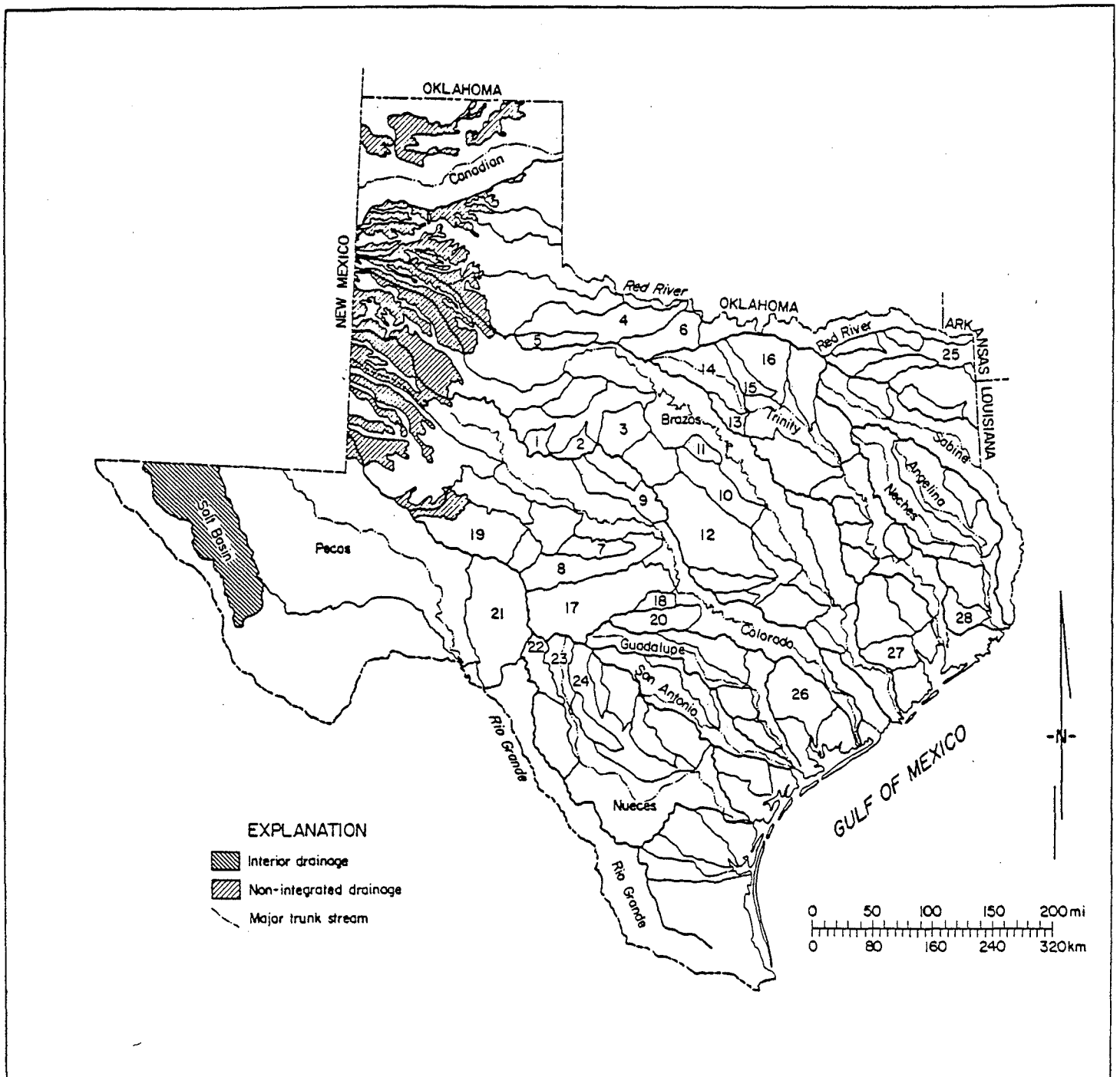
Figure 6. Generalized drainage basins of Texas. Selected basins denoted are: 1--Sweetwater Creek; 2--Elm Creek; 3--Hubbard Creek; 4--Wichita River; 5--South Wichita River; 6--Little Wichita River; 7--Brady Creek; 8--San Saba River; 9--Pecan Bayou; 10-- Bosque River; 11-- Paluxy River; 12--Leon/Lampasas Rivers; 13--Clear Fork of Trinity River; 14--West Fork of Trinity River; 15--Denton Creek; 16--Elm Fork of Trinity River; 17--Llano River; 18--Sandy Creek; 19--Middle Concho River; 20--Pedernales River; 21--Devils River; 22--West Nueces River; 23--Nueces River; 24--Frio River; 25--Sulphur River; 26--Lavaca/Navidad Rivers; 27-- Buffalo Bayou; 28--Pine Island Bayou.
