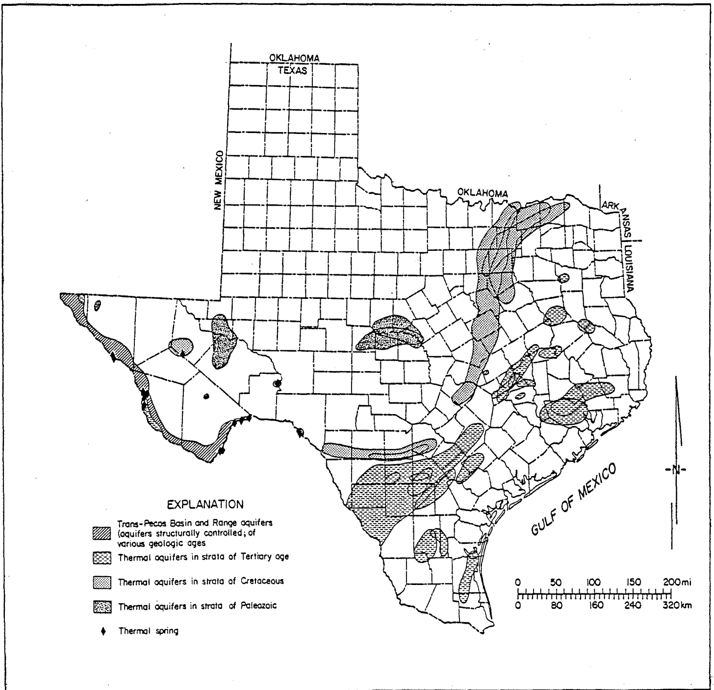
Figure 10. Simplified map showing extent of major geothermal aquifers and selected thermal springs in Texas.
