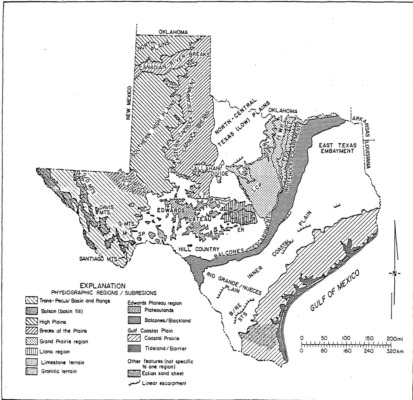
Figure 7. Generalized physiography of Texas. Selected areas abbreviated on map are: B/RE--Bordas/Reynosa Escarpment; ECT--Eastern Cross Timbers; EFP--Eagle Ford Prairie; ER--Enchanted Rock; Ft. WP--Fort Worth Prairie; G Mts.--Glass Mts.; G/D Mts.--Guadalupe/Delaware Mts.; LCP--Lampasas Cut Plain; LF--Lipan Flat; M--Marathon Area; PDC--Palo Duro Canyon; SB--Salt Basin; SP--Stockton Plateau; STS--South Texas Salient; WCT--Western Cross Timbers.
