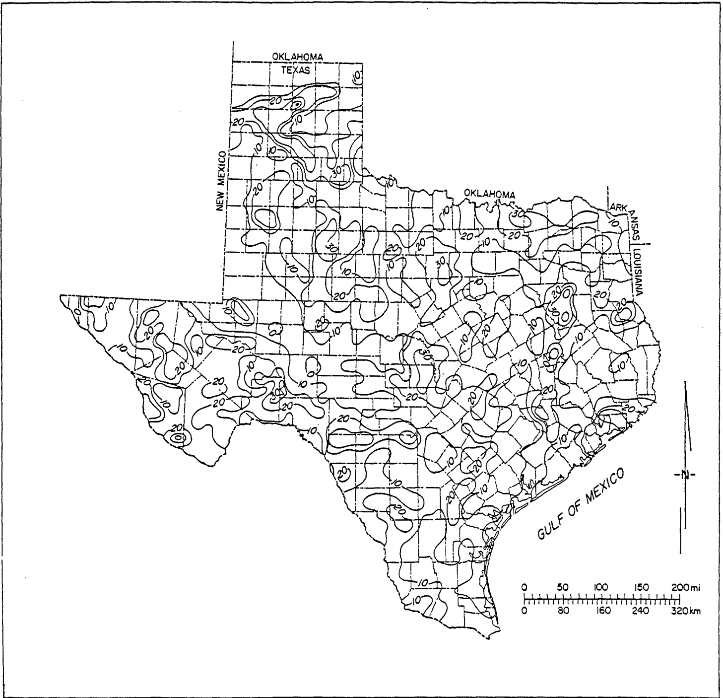
Figure 3. Number of lineaments per unit area (249 mi 2 or 645 km 2 ) without a moving average.
