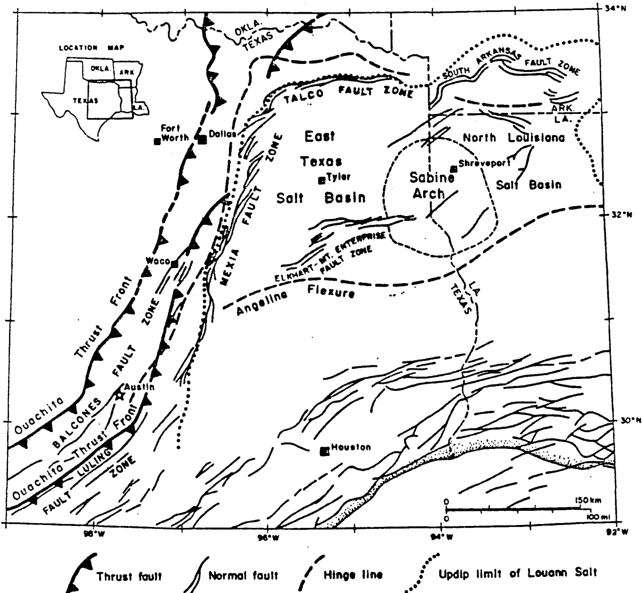
Figure 2. Regional tectonic setting of the East Texas Basin. Position of Angeline Flexure is mapped at base of Austin Chalk. Adapted from Martin (1978).
