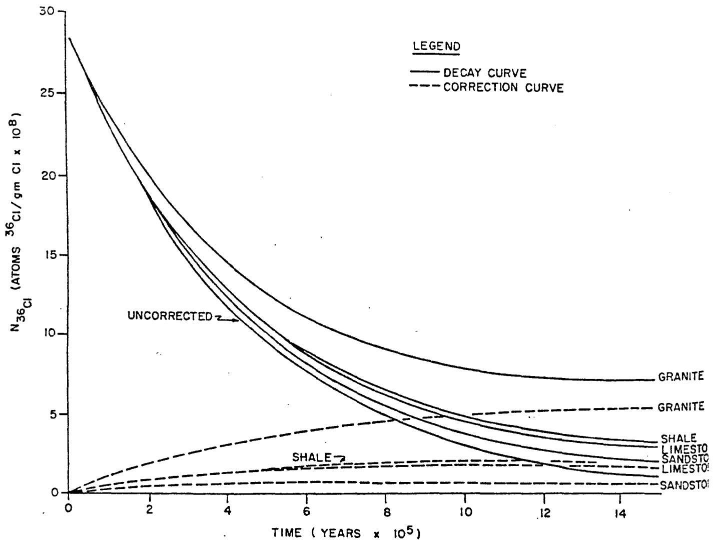
21 Figure 7 Decay curve of representative ^{36}Cl groundwater samples from different aquifers. The curves rising with time represent the subsurface contribution to ^{36}Cl as a function of aquifer type; the decay curves assume an initial concentration of 2.8 \times 10^9 atoms ^{36}Cl/gmCl (atmospheric component) and 1 \times 10^8 atoms ^{36}Cl/gmCl (soil surface component).
