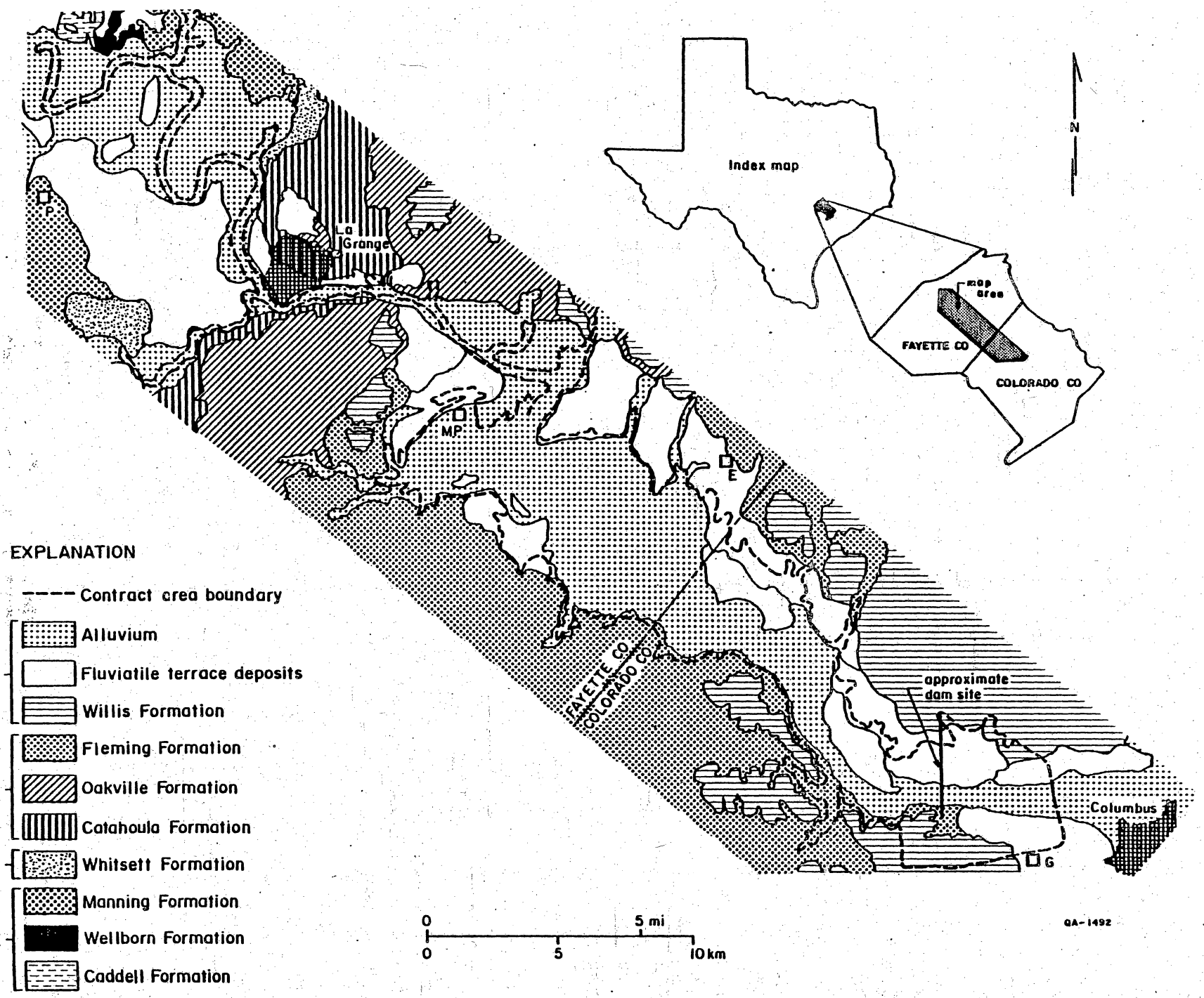
Figure 1. Geologic map of the proposed Columbus Bend reservoir site (contract area) (from Barnes, 1974) (P = Plum, MP = Mullins Prairie, E = Ellinger, G = Glidden).
