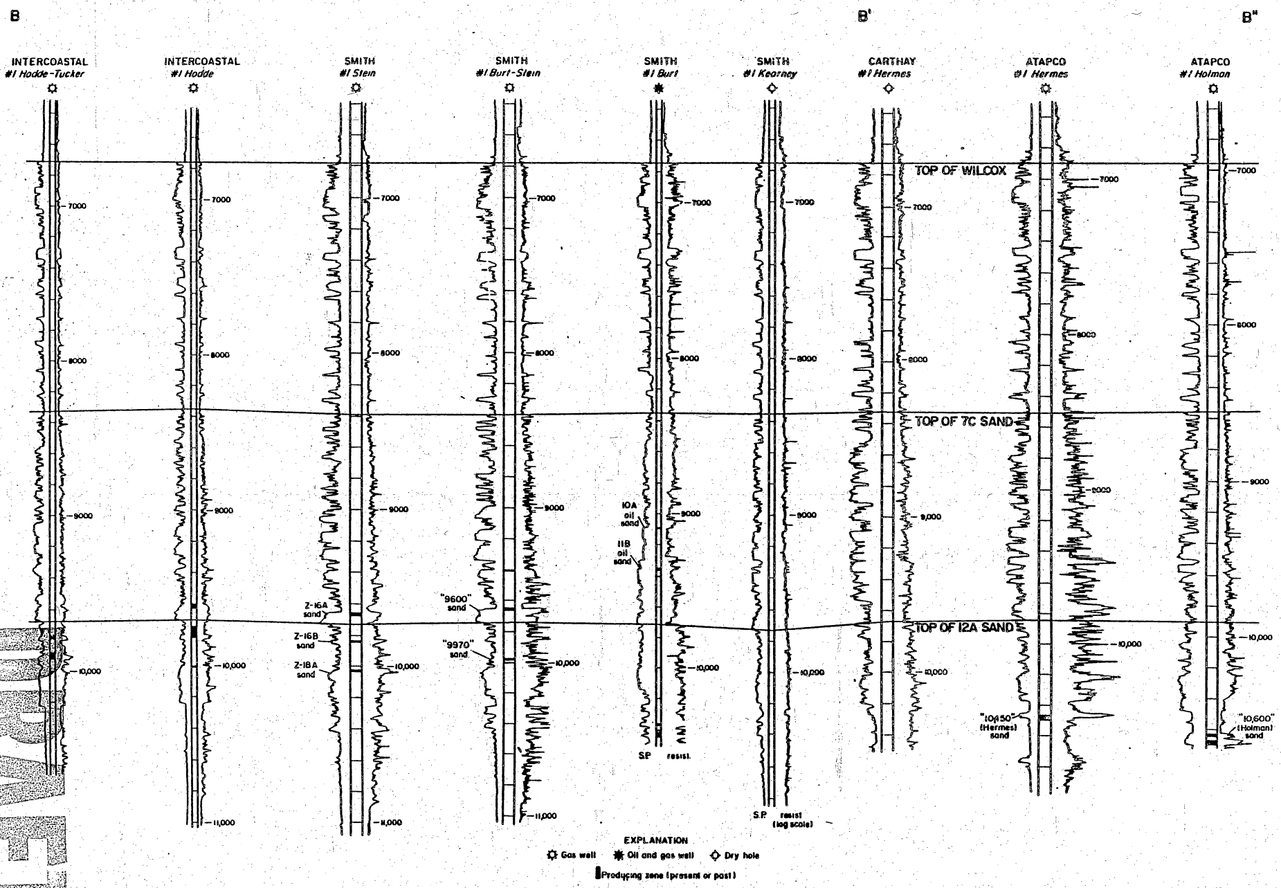
Figure 8. Strike (B-B') and dip (B'-B'') cross sections through the Columbus West and Glidden fields. Location of section shown on figure 6. Not to horizontal scale.
