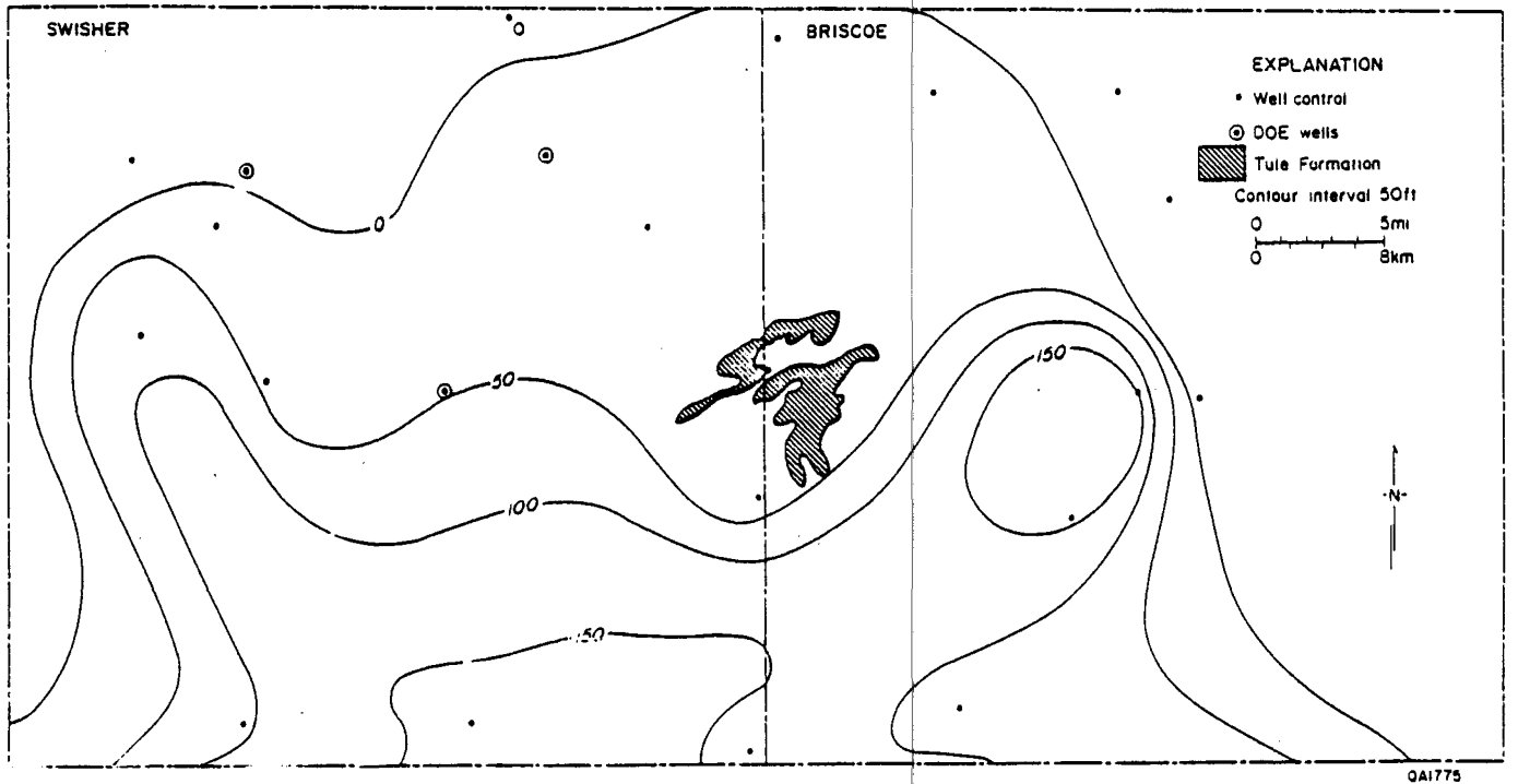
Figure 11. Net-salt map for the Upper Permian Salado Formation, Swisher and Briscoe Counties.
