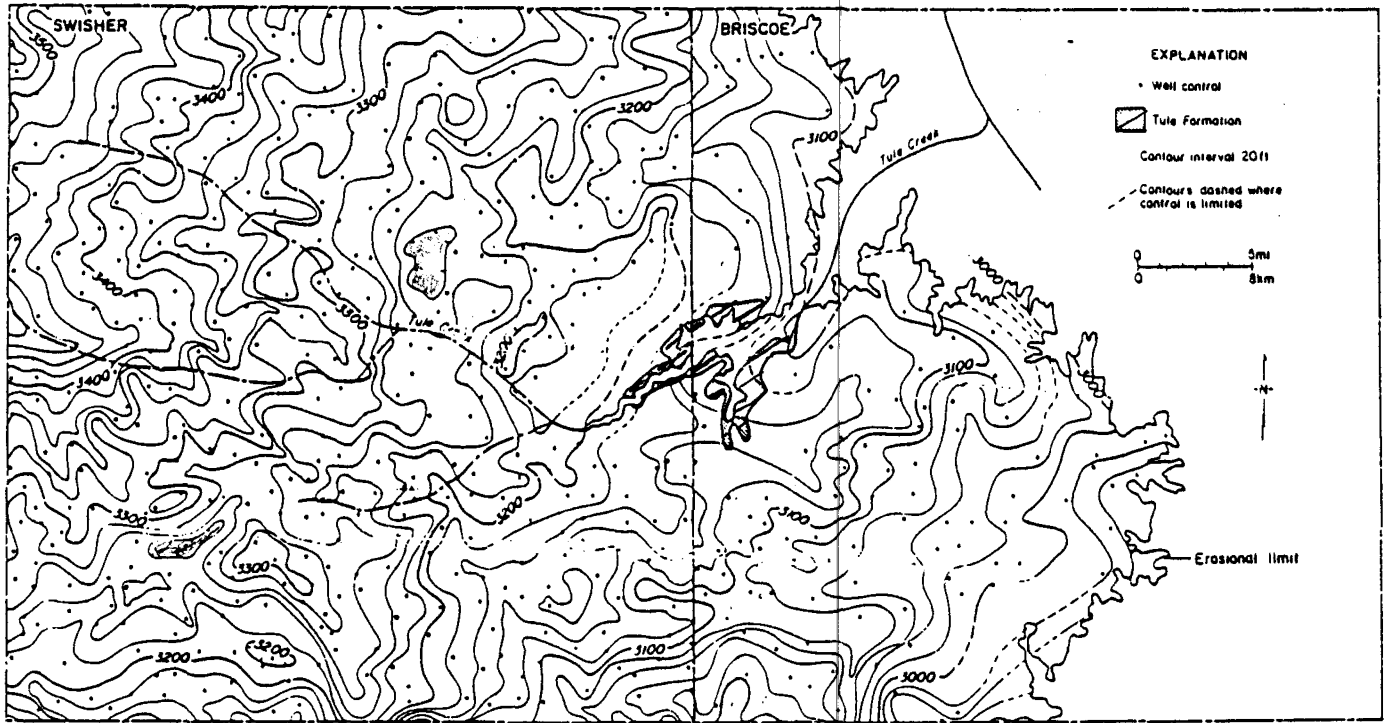
Figure B13 Paleotopography on the middle Tertiary erosion surface (base of the High Plains Aquifer), Swisher and Briscoe Counties (after Knowles and others, 1982).
