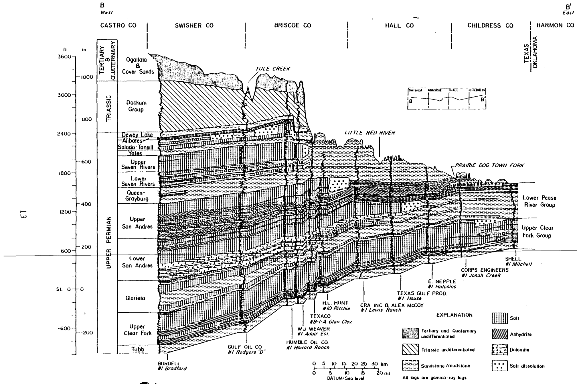
Figure 3. Stratigraphic cross section showing Upper Permian, Triassic, Tertiary and Quaternary strata. Salt dissolution is illustrated between wells where some or all of the salt section is missing and where structural collapse of strata has occurred.
