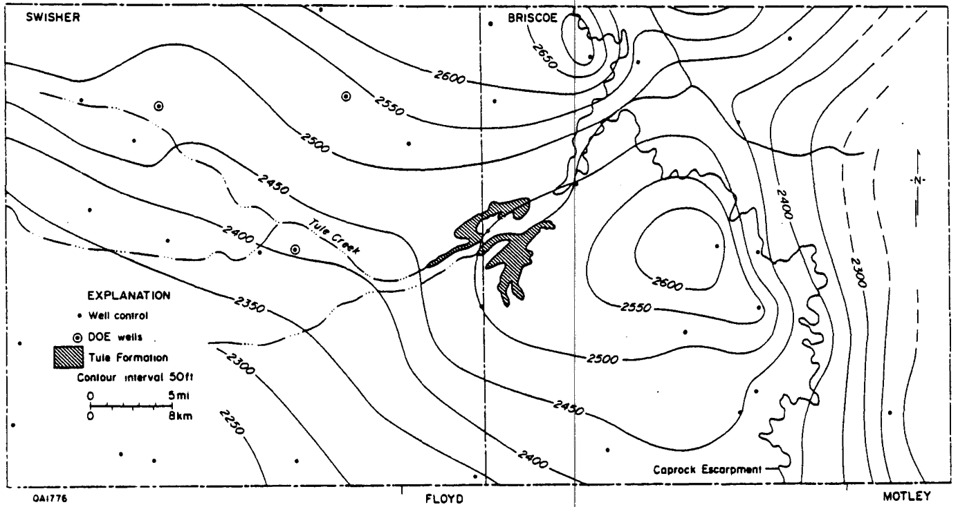
Figure 12. Structure-contour map on the top of the Upper Permian Alibates Formation, Swisher and Briscoe Counties.
