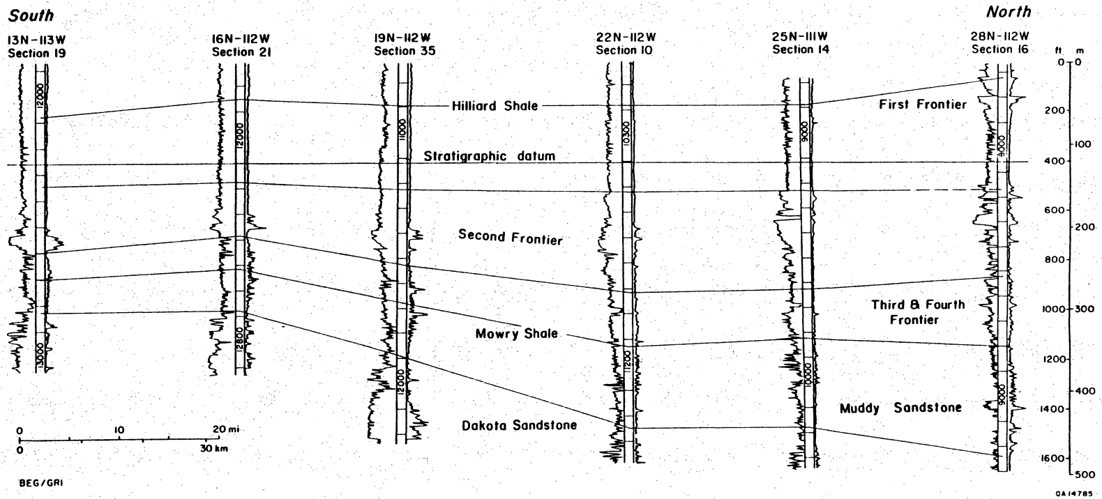
Figure 4. Regional north-south, gamma-ray/resistivity cross section along the Moxa Arch (from Dutton and Hamlin, 1991). Line of section shown in fig. 1.
