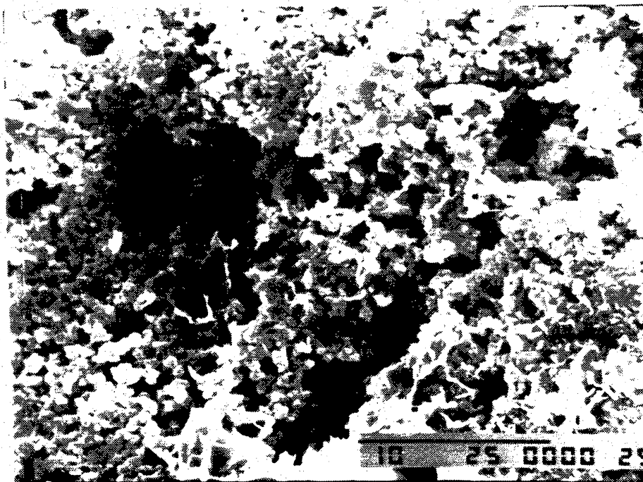
Figure 18. Close-up of surface of chert grain shown in figure 17. Partial dissolution of chert has resulted in abundant micropores. SEM photo by K. L. Herrington. Scale bar is 10 \mu\text{m} .
