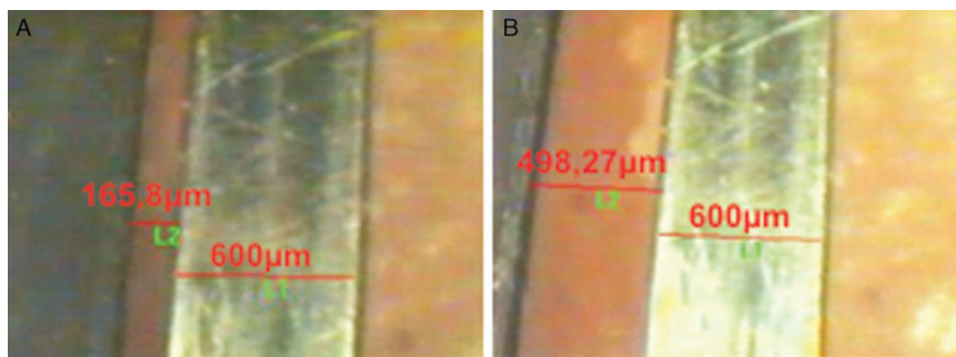
Figure 2 (A) The reference strip before applying the load; and (B) during application of the load.
