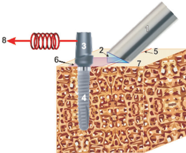
Figure 1 (1) Contact endoscope; (2) field of vision; (3) screw; (4) dental implant; (5) reference wire; (6) indicator strip; (7) sample of bone; (8) lateral load.
